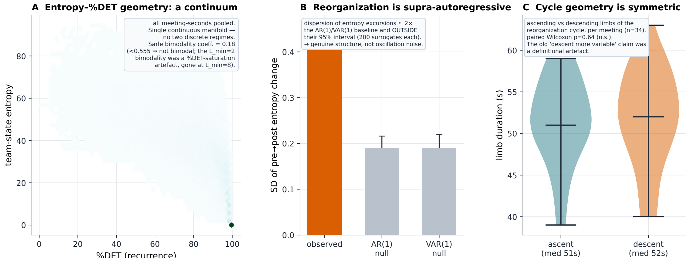
Figure 2. (A) Pooled across all meeting-seconds, entropy and %DET form one continuous manifold — not two discrete coordination regimes (Sarle bimodality coefficient below the 0.555 threshold; the earlier bimodality was a %DET-saturation artefact removed by L_{\min}=8 ). (B) The dispersion of pre→post entropy excursions at reorganization is \sim 2\times and outside the 95% interval of AR(1) and VAR(1) surrogates (200 each) — genuine structure beyond trivial oscillation. (C) Ascending and descending limbs of the cycle are symmetric (paired Wilcoxon, n.s.).
