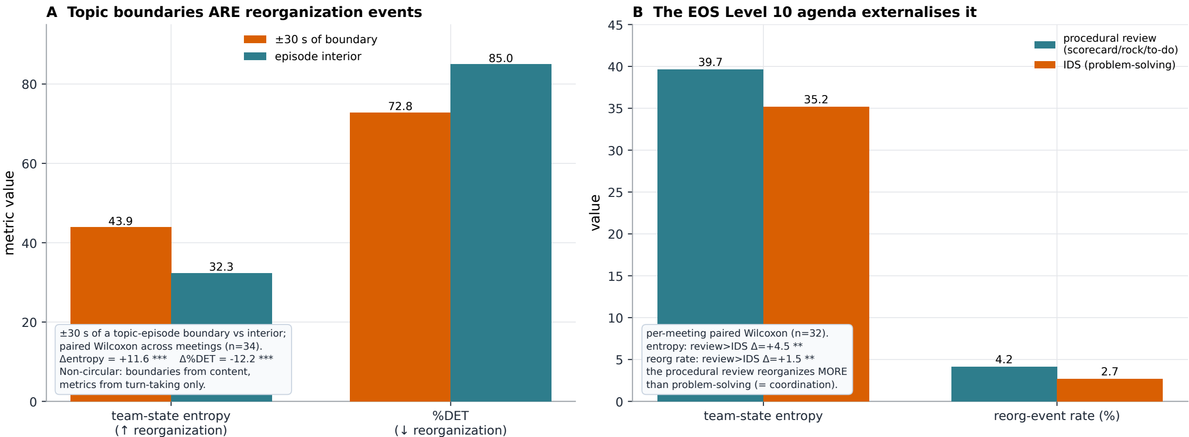
Figure 6. (A) In \pm 30 s of a topic-episode boundary, team-state entropy rises and %DET falls vs episode interiors — topic transitions are the naturalistic perturbation that drives reorganization (non-circular: boundaries are lexical, metrics are turn-taking). (B) On the EOS Level 10 agenda these teams run, the procedural review stages reorganize more than the problem-solving (IDS) block — reorganization is coordination, not deliberation. Paired Wilcoxon; * p < .05 , ** p < .01 , *** p < .001 .
