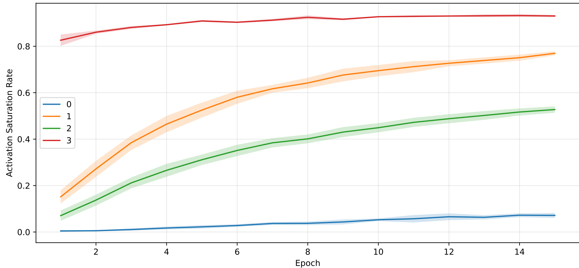
Tanh - Activation Saturation Rate Curve (Mean and Std over Trials)
