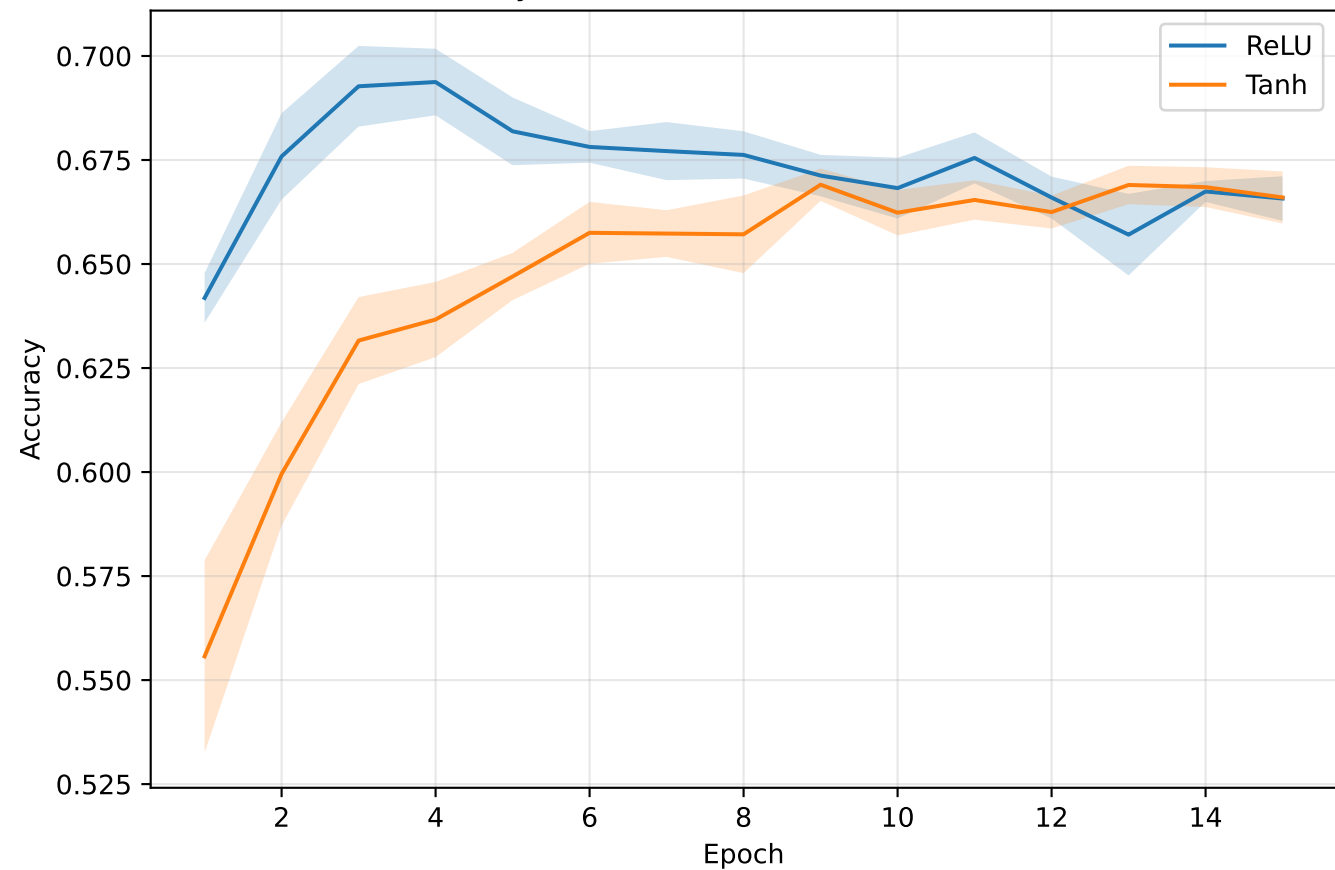
Accuracy Curve (Mean and Std over 5 Trials)
