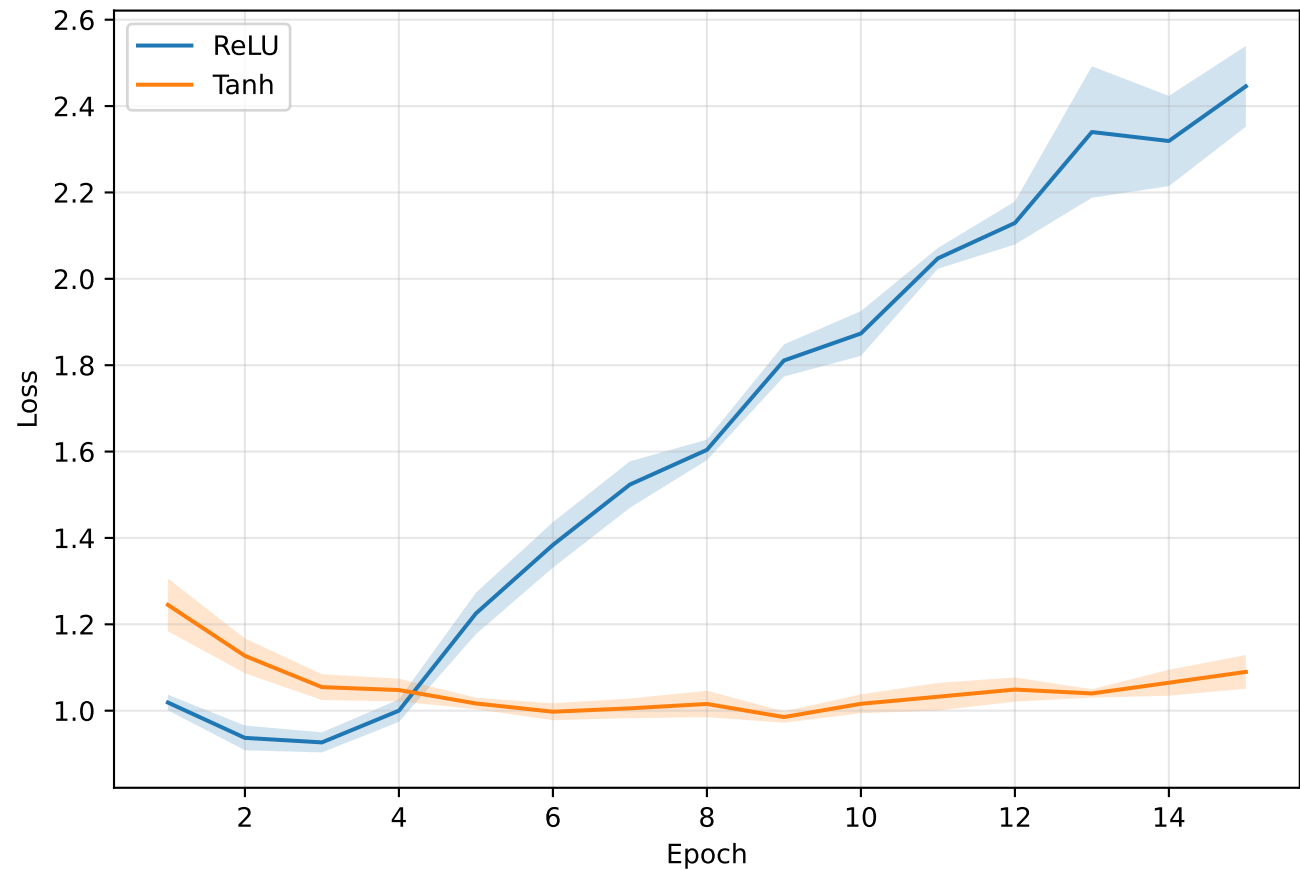
Loss Curve (Mean and Std over 5 Trials)
