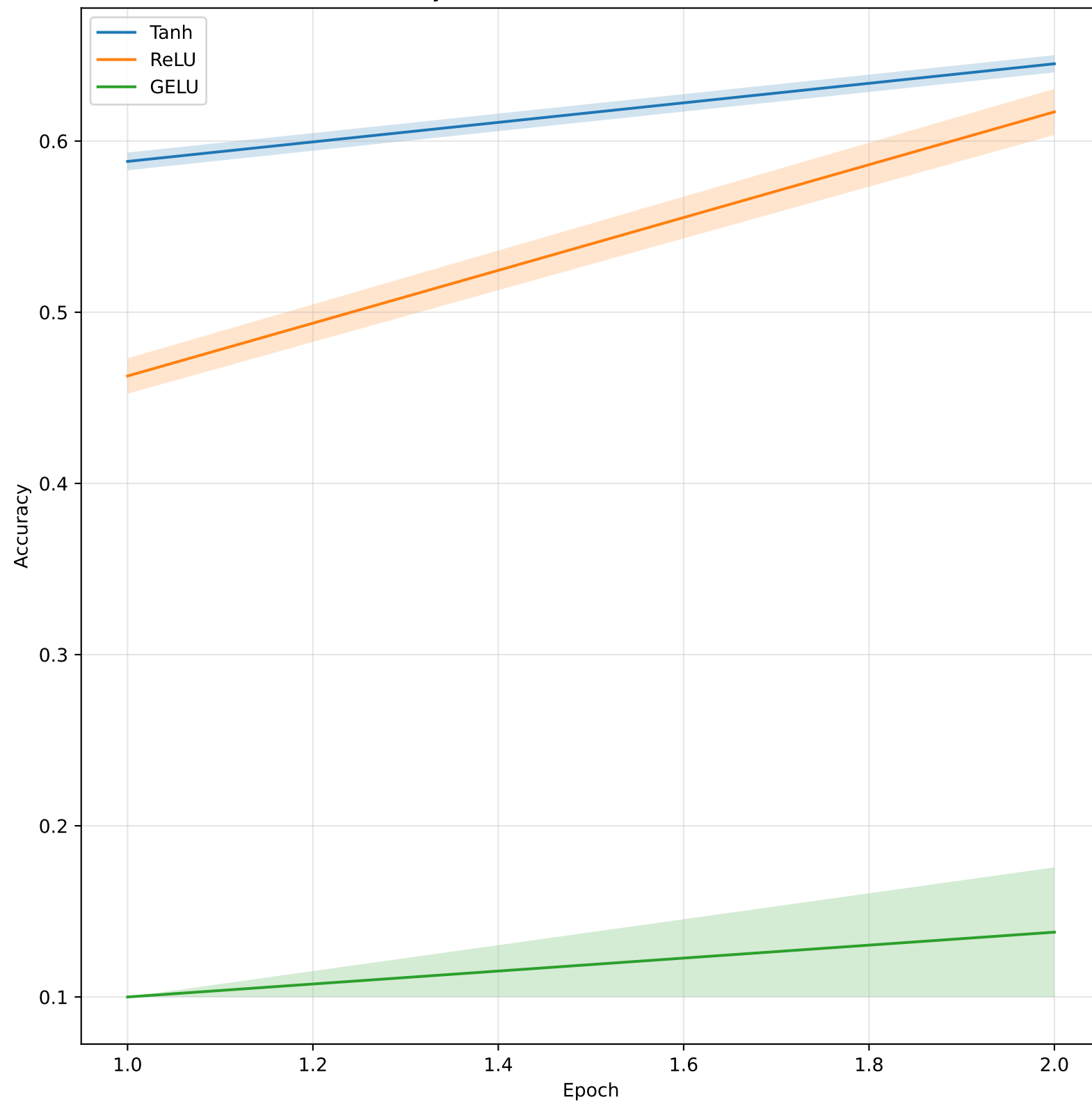
Accuracy Curve (Mean and Std over 5 Trials)
