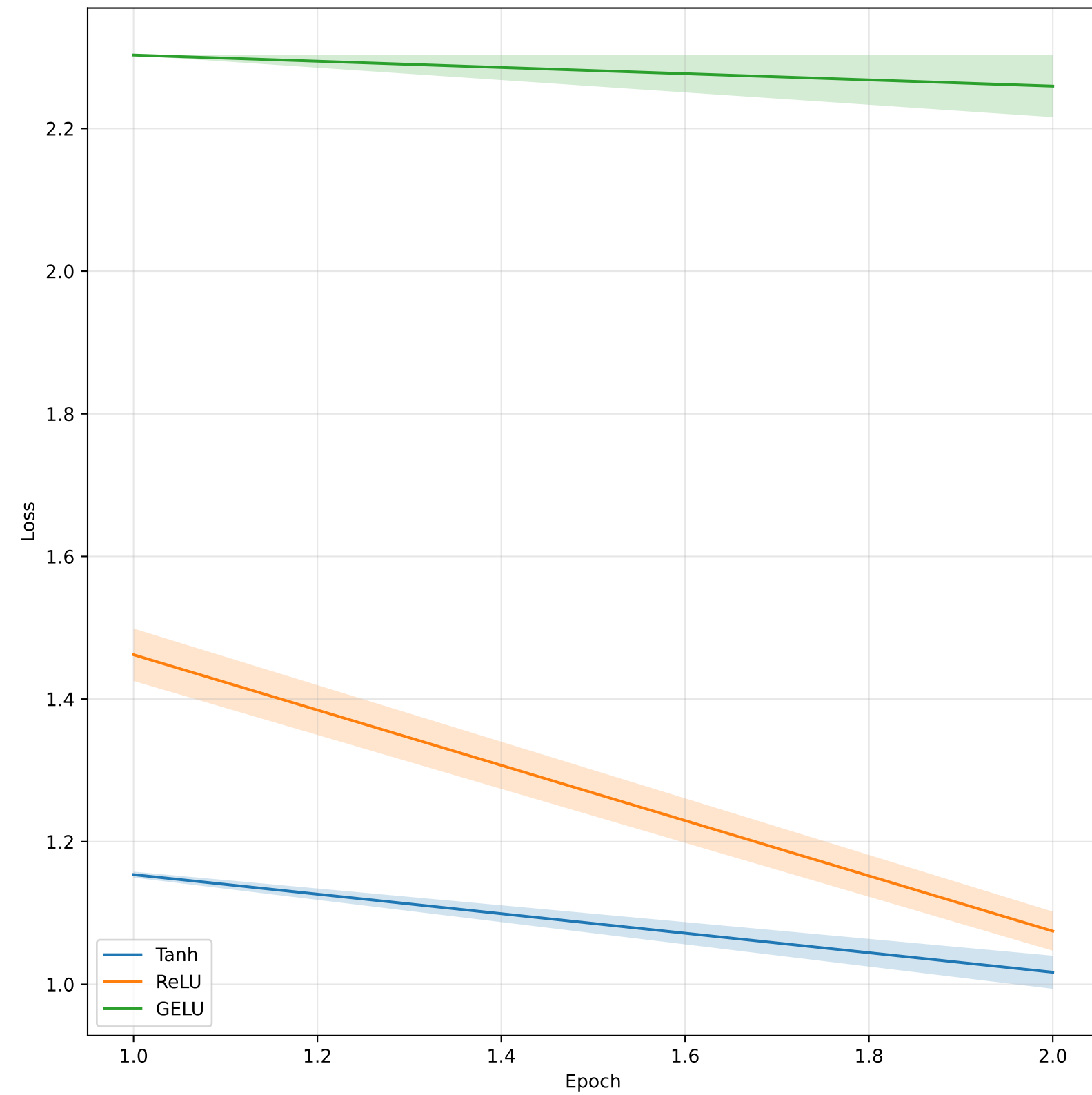
Loss Curve (Mean and Std over 5 Trials)
