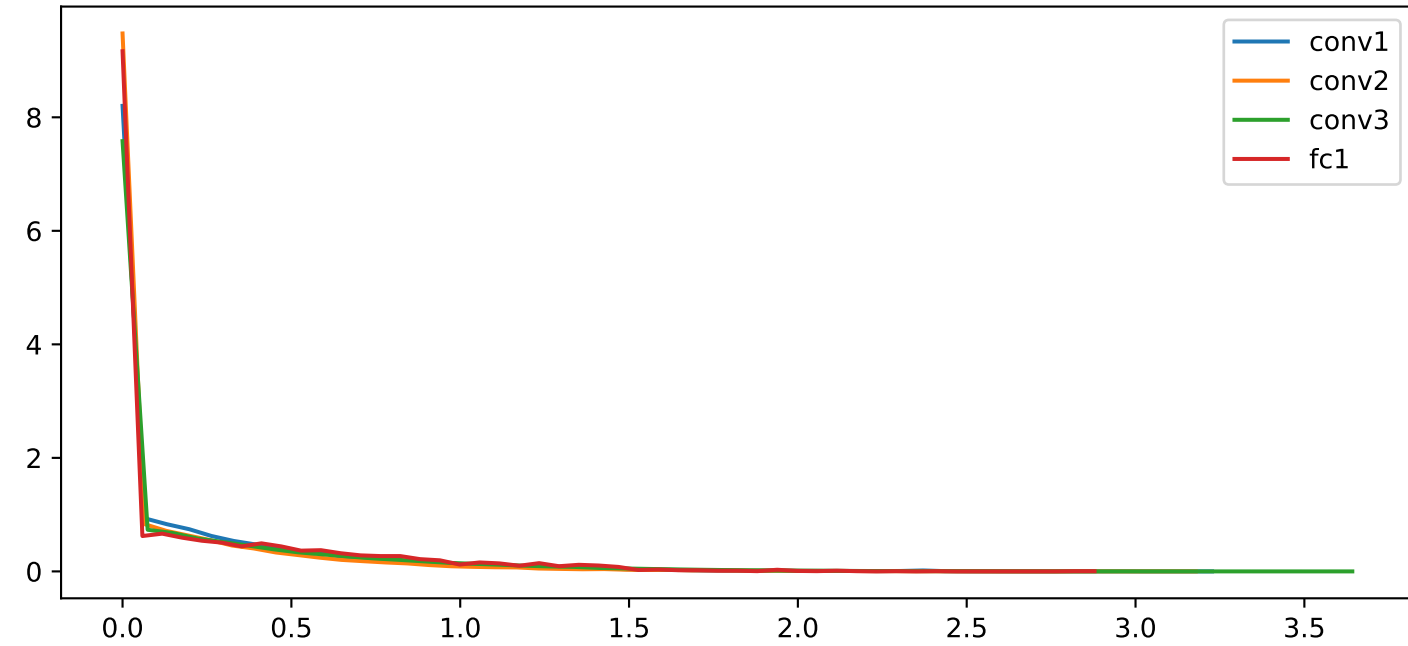
Activation distributions - ReLU
