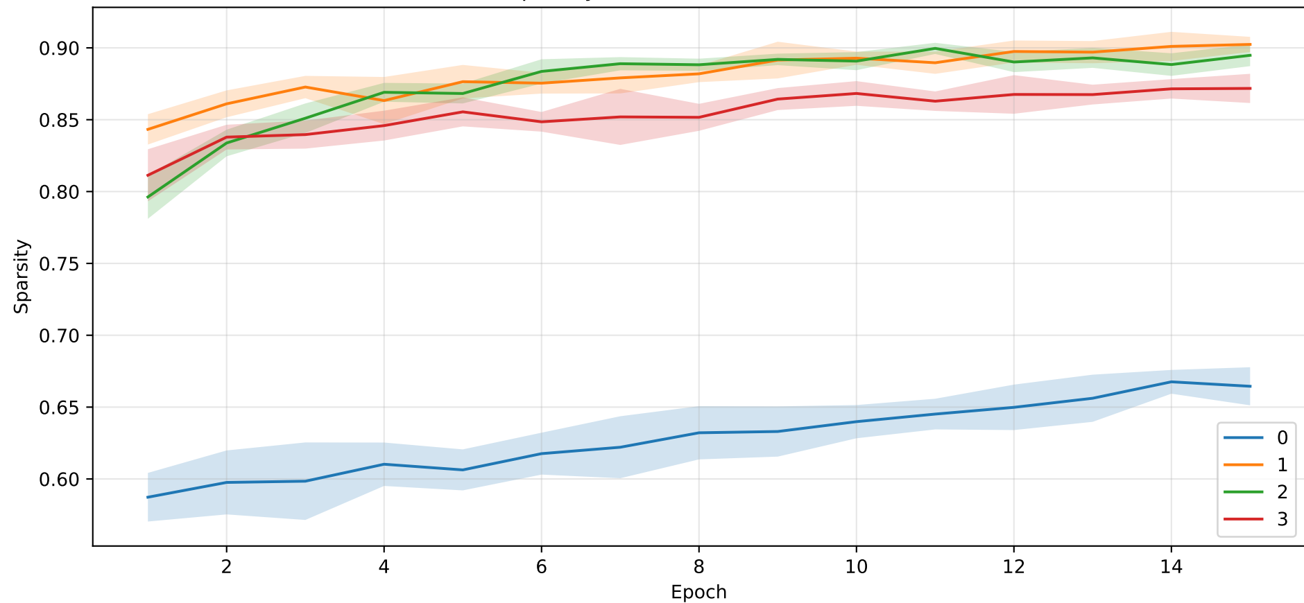
ReLU - Sparsity Curve (Mean and Std over Trials)
