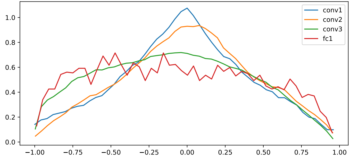
Activation distributions - Tanh
