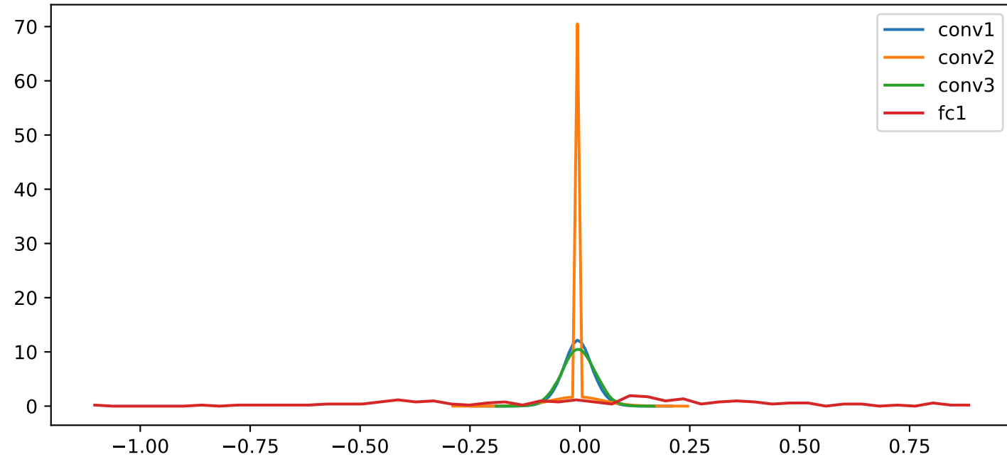
Gradient distributions - Tanh
