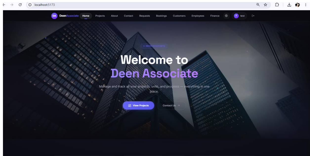
Figure 1: Home Page
