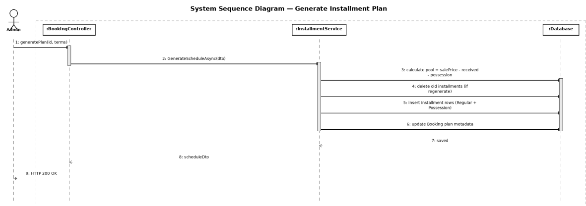
Figure 3.9: Admin generates installment schedule for booking
