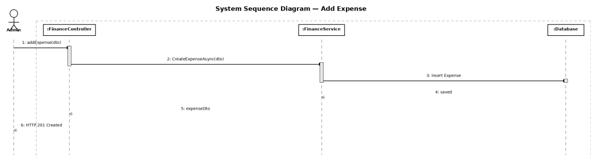
Figure 3.18: Admin adds expense entry to finance ledger
