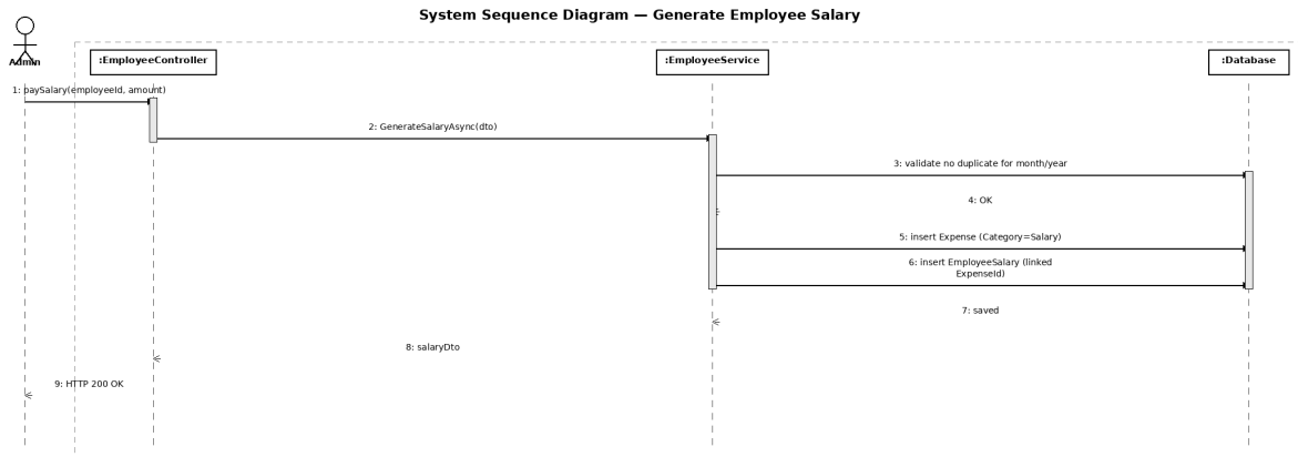
Figure 3.15: Admin generates salary payment and linked expense
