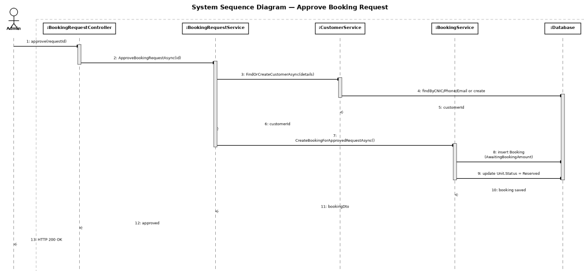
Figure 3.5: Admin approves request and creates confirmed booking
