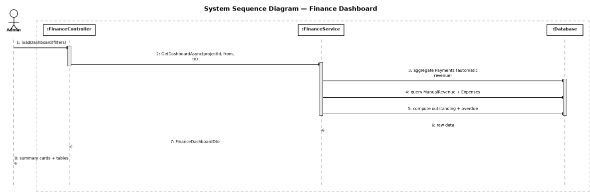
Figure 3.16: Admin loads financial summary and transaction lines
