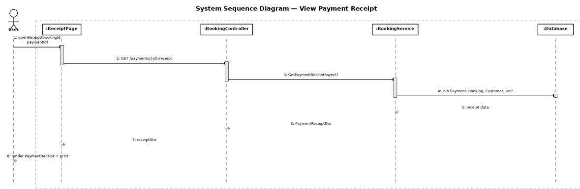
Figure 3.11: Admin or Client views printable payment receipt
