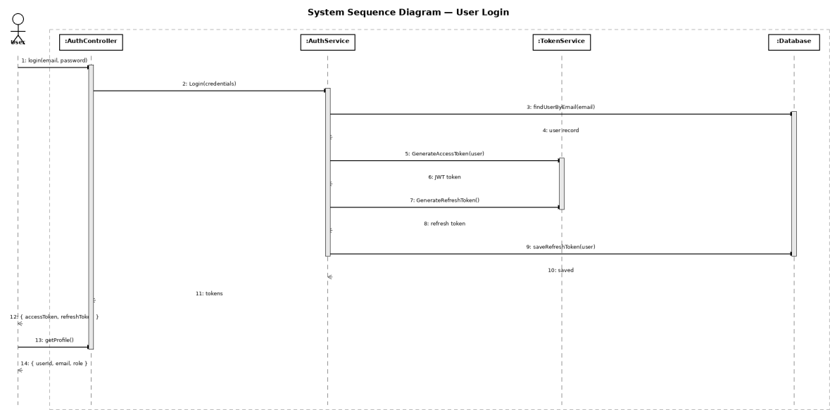
Figure 3.2: User Login and profile load
