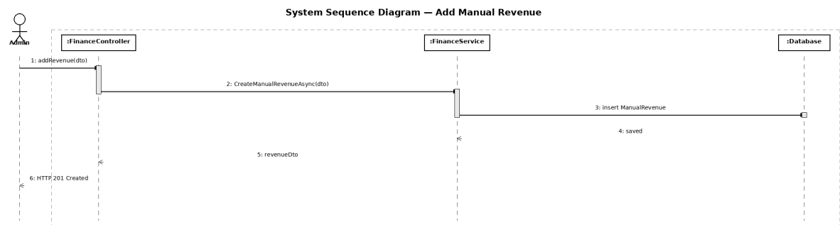
Figure 3.17: Admin adds manual revenue entry to finance ledger
