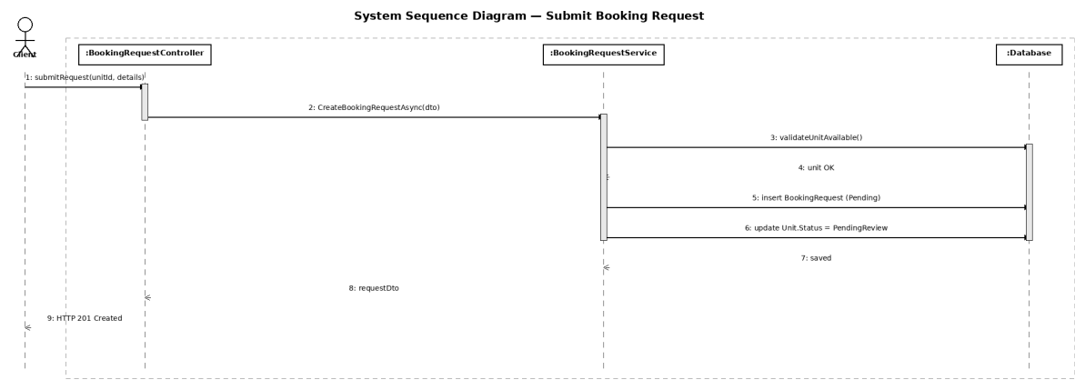
Figure 3.4: Guest/Client submits booking request for a unit
