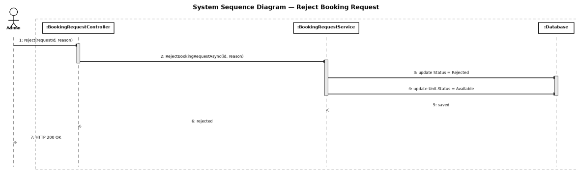
Figure 3.6: Admin rejects booking request and releases unit
