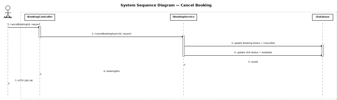
Figure 3.13: Admin cancels booking and releases unit
