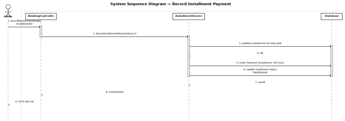
Figure 3.10: Admin records installment payment and generates receipt
