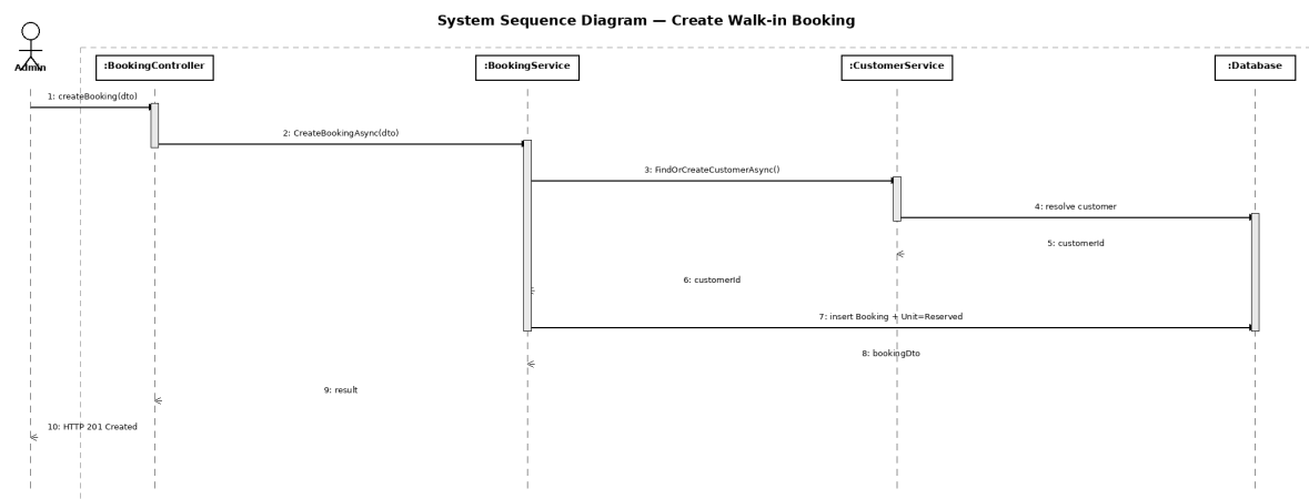
Figure 3.7: Admin creates direct booking for walk-in customer
