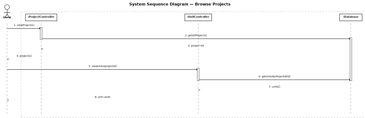
Figure 3.3: Guest browses projects and units
