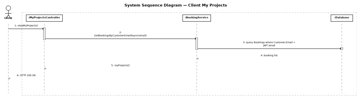
Figure 3.12: Client views own confirmed bookings by email match
