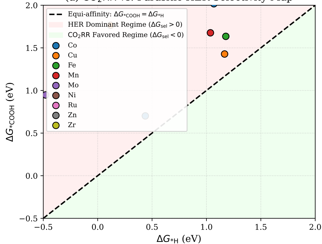
(a) CO 2 RR vs. Parasitic HER Selectivity Map
