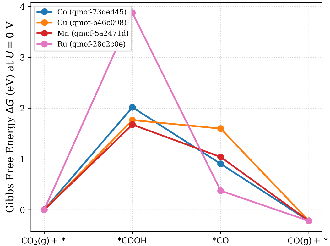
(b) CO 2 RR ( \text{C}_1 \rightarrow \text{CO} ) Free Energy Profiles
