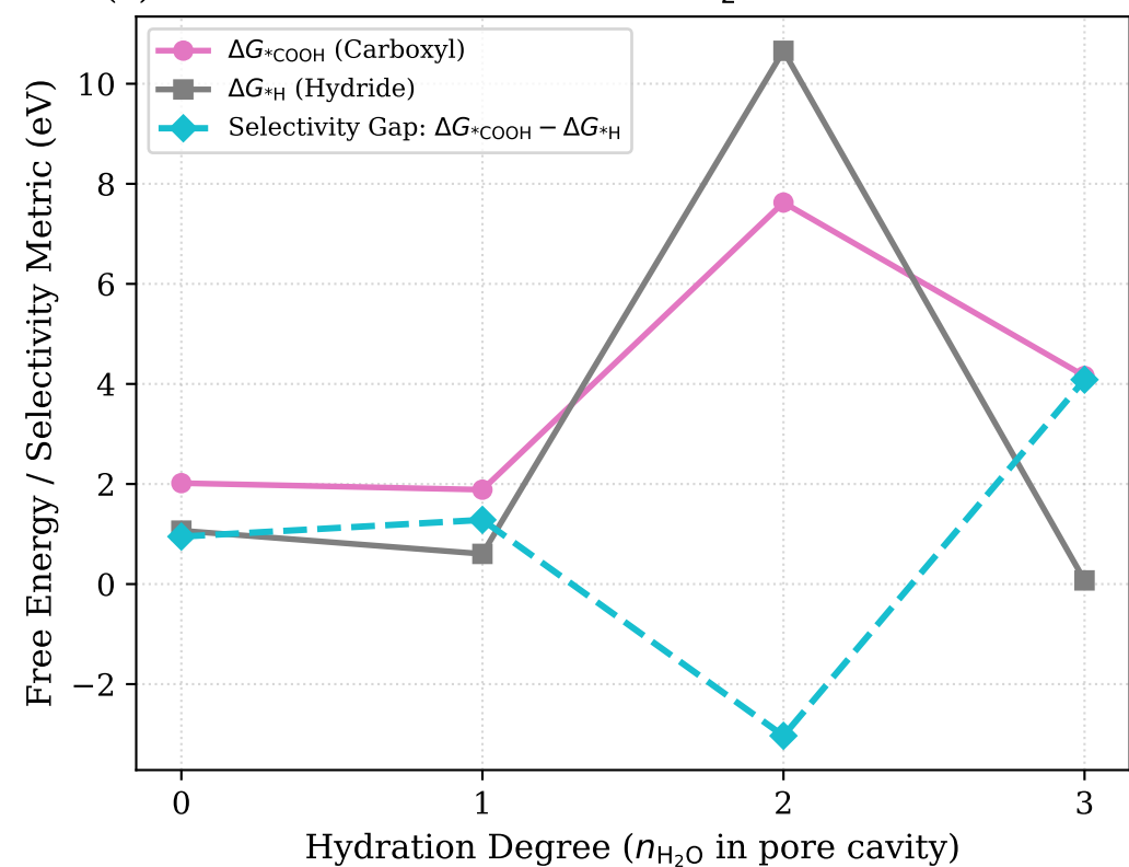
(c) Selective Solvation Favors CO 2 RR Over Parasitic HER
