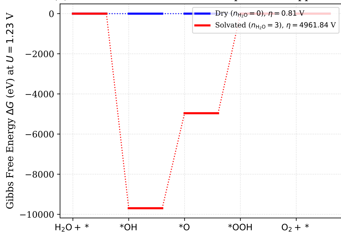
(b) Co-MOF-74 OER Profiles: Overpotential Suppression
