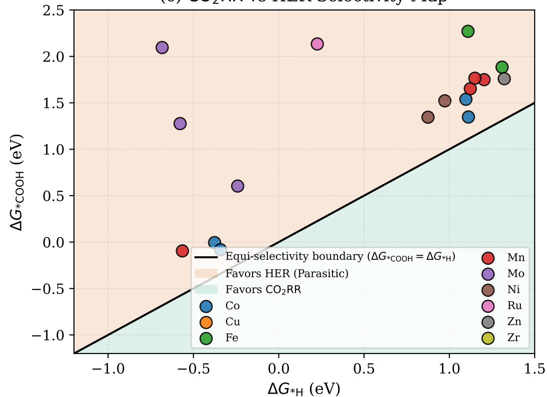
(c) CO 2 RR vs HER Selectivity Map
