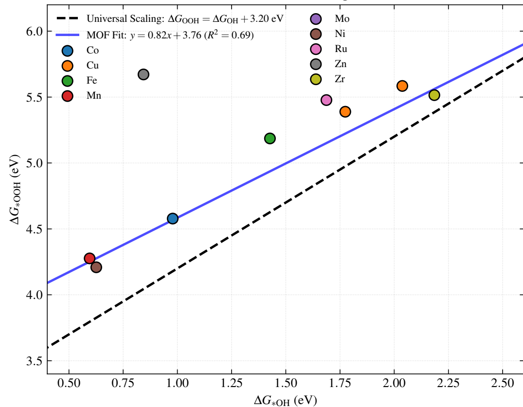
(a) OER Intermediate Scaling Relation
