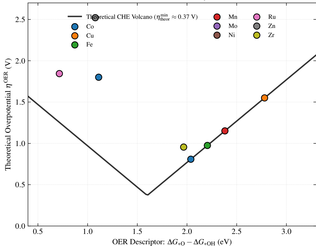
(b) OER Volcano Activity Curve
