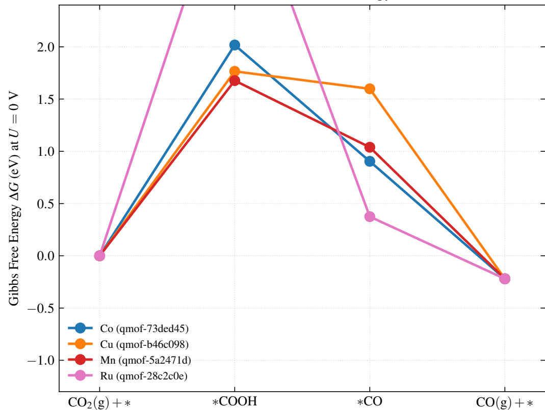
(b) CO 2 RR (C 1 → CO) Free Energy Profiles
