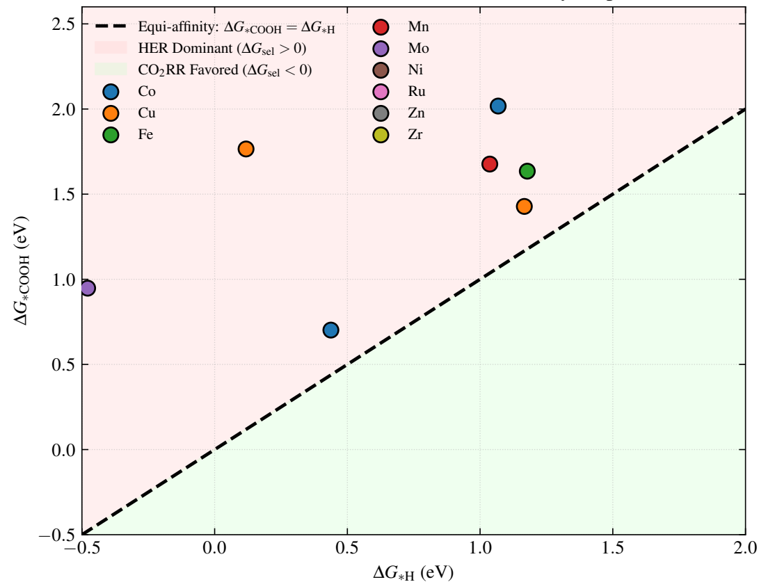
(a) CO 2 RR vs. Parasitic HER Selectivity Map
