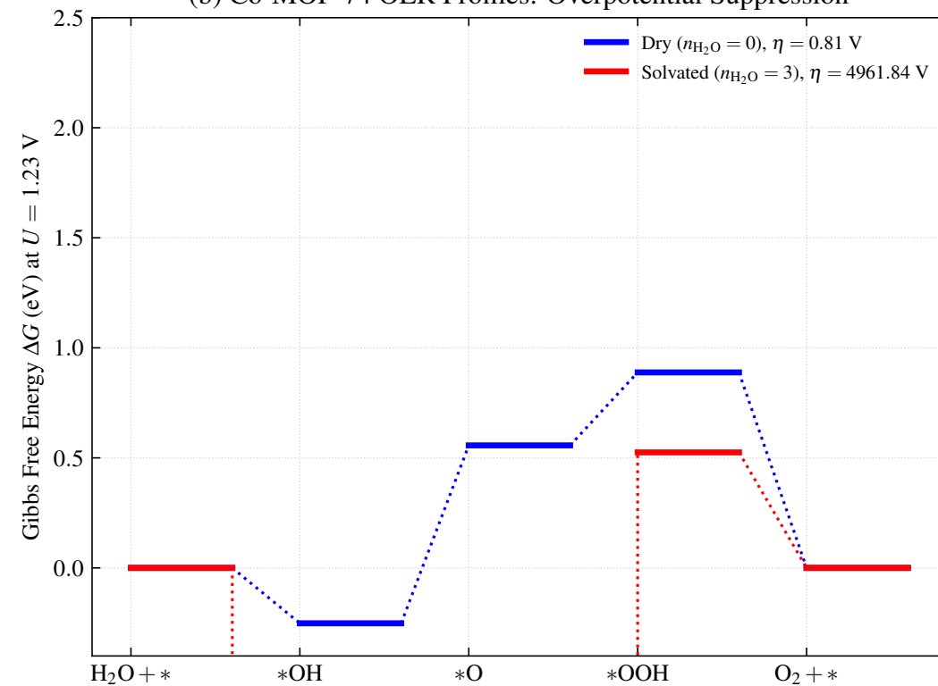
(b) Co-MOF-74 OER Profiles: Overpotential Suppression
