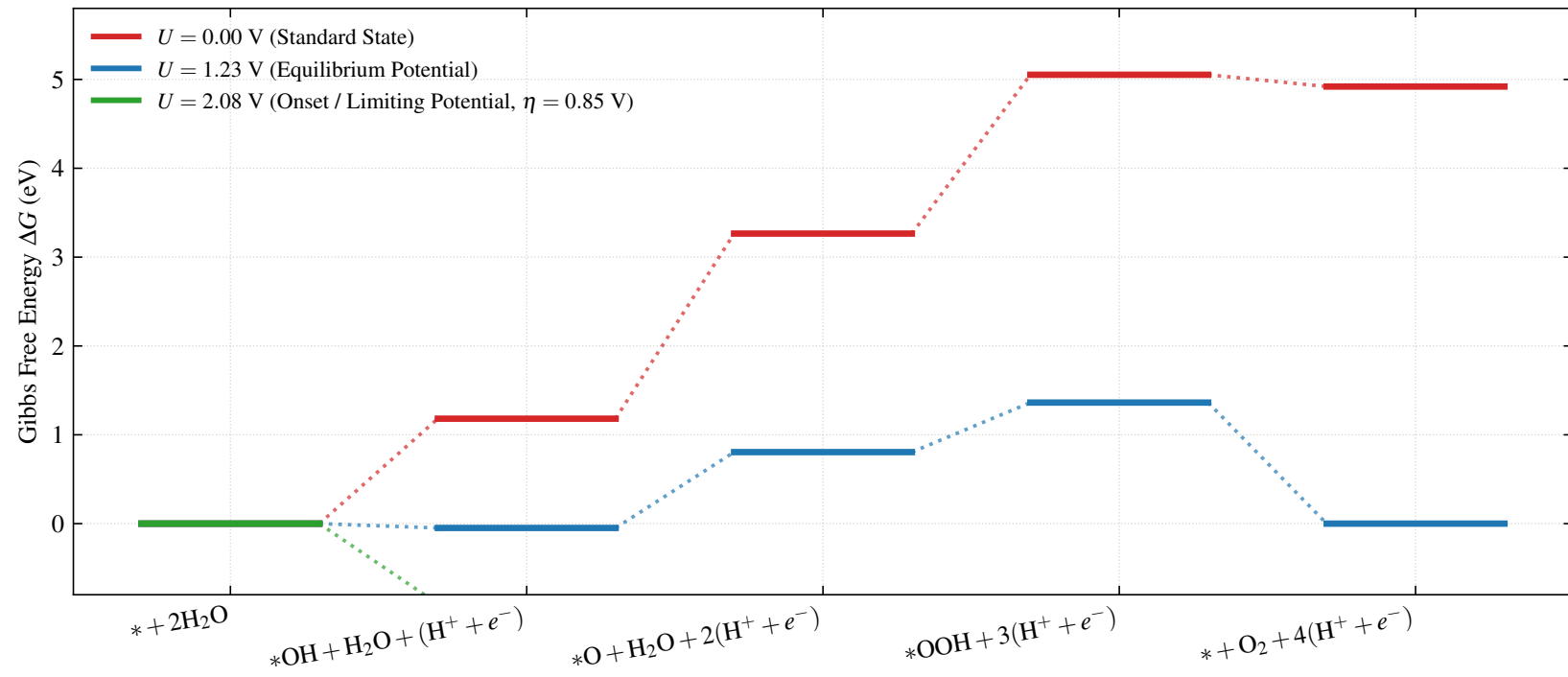
OER Reaction Coordinate: Co-MOF (qmof-73ded45)
