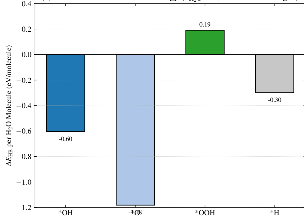
(d) Pore H-Bond Stabilization Energy ( n_{H_2O} = 1 , 4/6 states converged)
