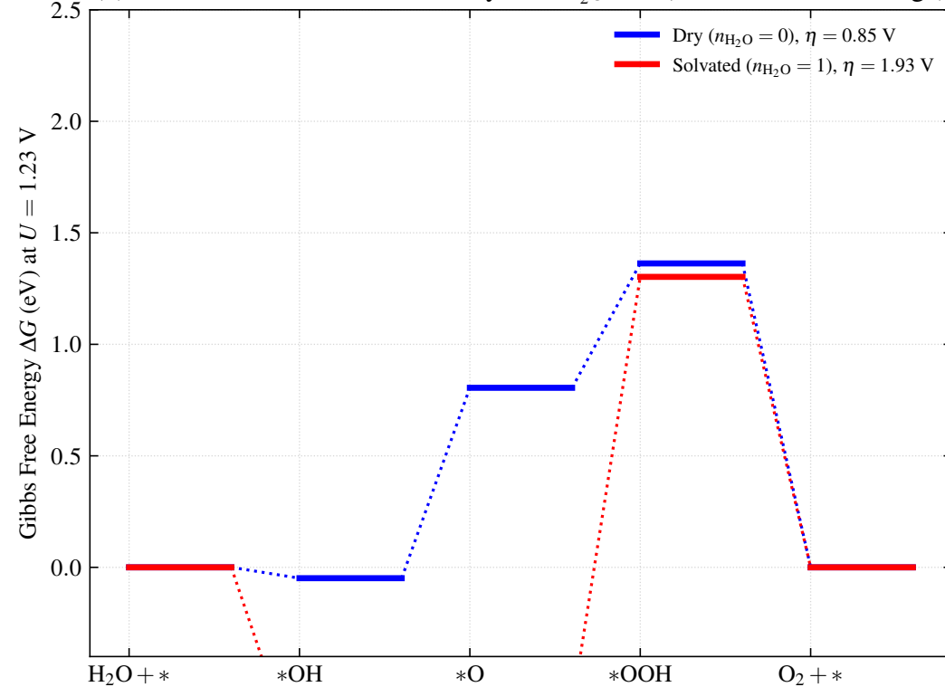
(b) Co-MOF-74 OER Profiles: Dry vs. n_{H_2O} = 1 ( n=2,3 did not converge)
