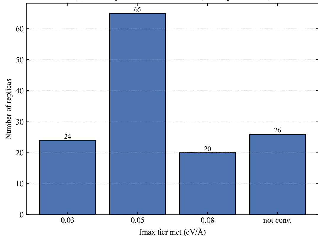
(b) Convergence-tier distribution (135 replicas total)
