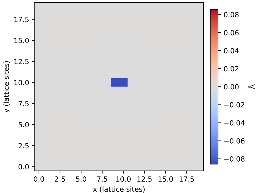
Holstein distortion u
