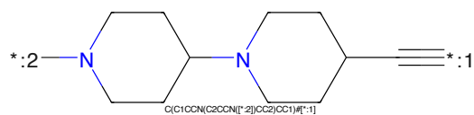
Figure 927: LINKER - PROTAC ID: 690
