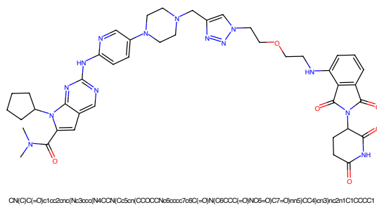
Figure 201: PROTAC - PROTAC ID: 436
