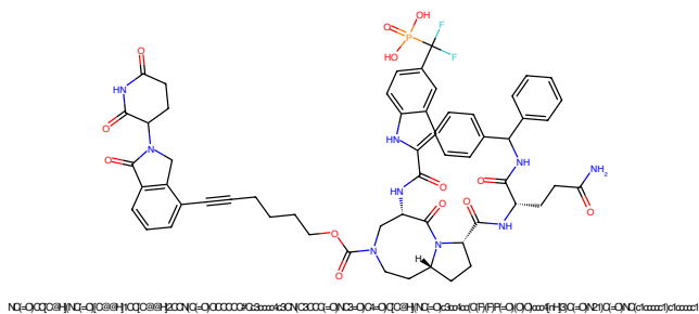
Figure 729: PROTAC - PROTAC ID: 627
