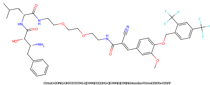
Figure 457: PROTAC - PROTAC ID: 509
