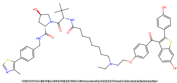
Figure 553: PROTAC - PROTAC ID: 542
