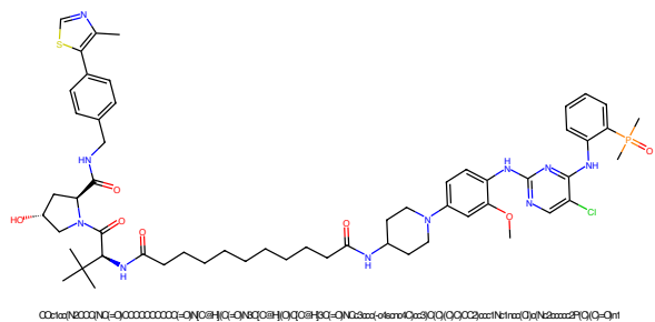
Figure 637: PROTAC - PROTAC ID: 565
