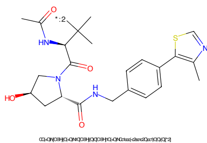
Figure 20: E3 - PROTAC ID: 354
