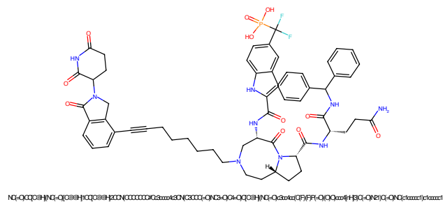
Figure 725: PROTAC - PROTAC ID: 626
