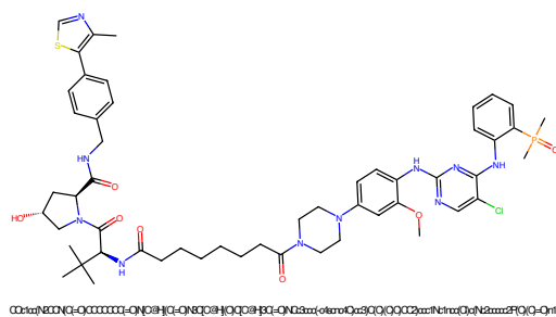
Figure 601: PROTAC - PROTAC ID: 556
