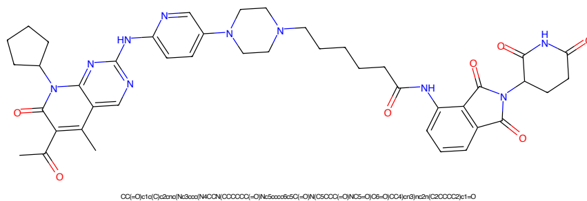
Figure 585: PROTAC - PROTAC ID: 551
