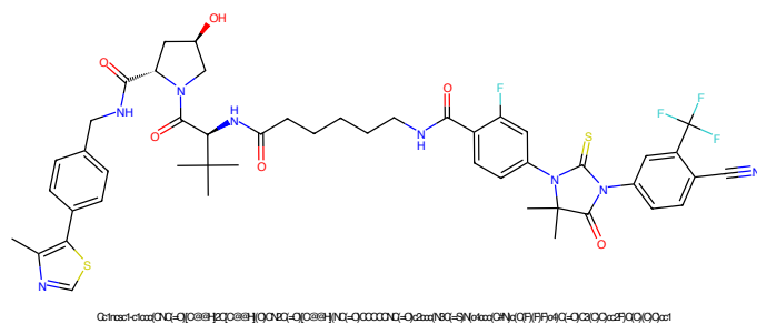
Figure 853: PROTAC - PROTAC ID: 662
