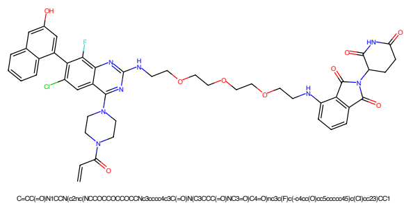
Figure 957: PROTAC - PROTAC ID: 698
