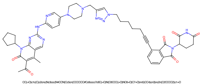
Figure 169: PROTAC - PROTAC ID: 428
