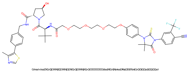
Figure 25: PROTAC - PROTAC ID: 356
