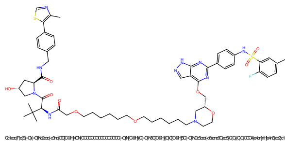
Figure 369: PROTAC - PROTAC ID: 486
