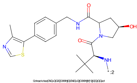
Figure 120: E3 - PROTAC ID: 414
