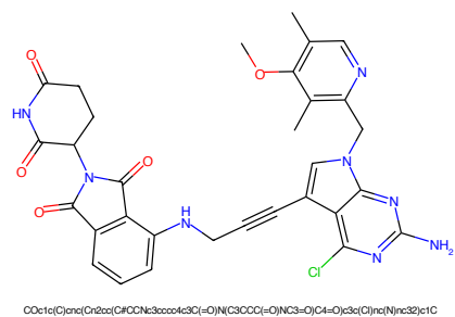
Figure 457: PROTAC - PROTAC ID: 3090
