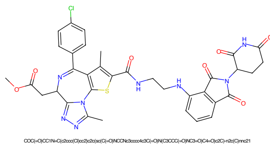
Figure 829: PROTAC - PROTAC ID: 1332
