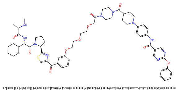
Figure 141: PROTAC - PROTAC ID: 2224
