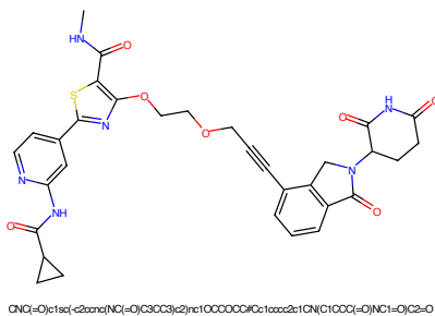
Figure 153: PROTAC - PROTAC ID: 2299
