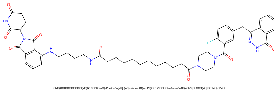
Figure 17: PROTAC - PROTAC ID: 2093
