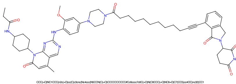
Figure 321: PROTAC - PROTAC ID: 2734
