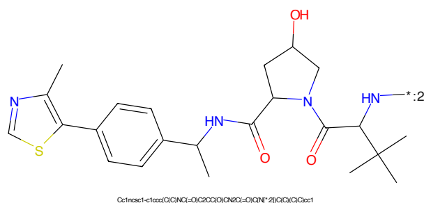
Figure 12: E3 - PROTAC ID: 1611
