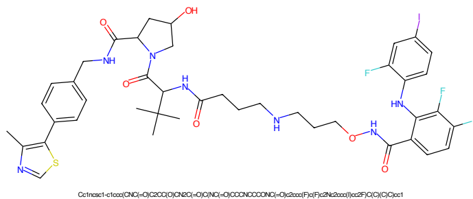
Figure 117: PROTAC - PROTAC ID: 2135
