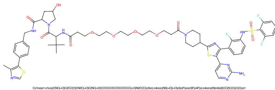
Figure 225: PROTAC - PROTAC ID: 2430
