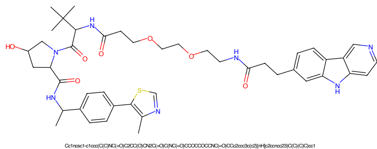
Figure 537: PROTAC - PROTAC ID: 3572
