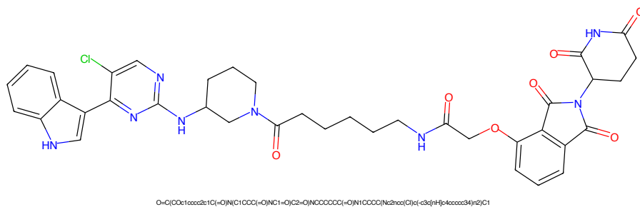
Figure 609: PROTAC - PROTAC ID: 2625
