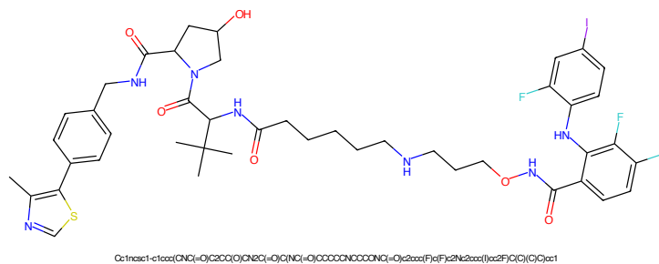
Figure 125: PROTAC - PROTAC ID: 2137
