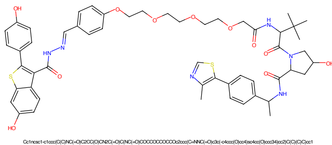
Figure 21: PROTAC - PROTAC ID: 1616
