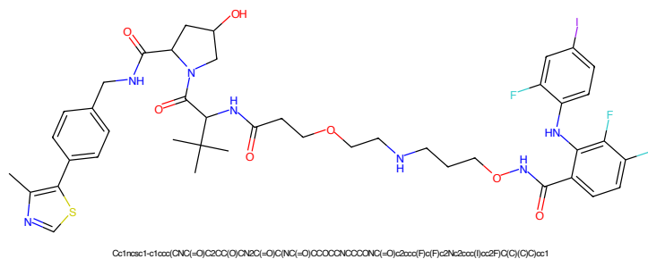
Figure 145: PROTAC - PROTAC ID: 2142
