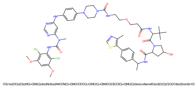
Figure 441: PROTAC - PROTAC ID: 3254
