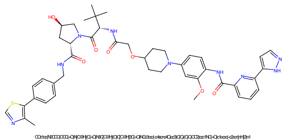
Figure 977: PROTAC - PROTAC ID: 3435
