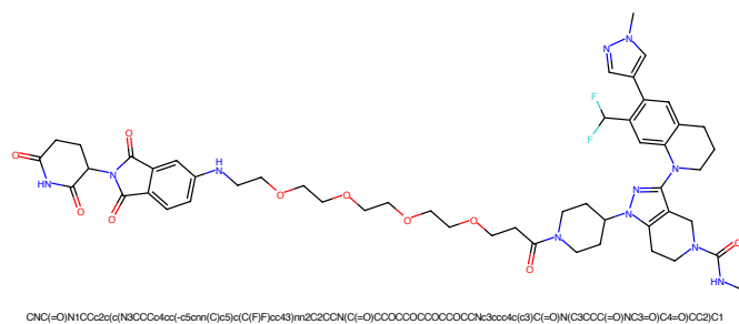
Figure 765: PROTAC - PROTAC ID: 2375
