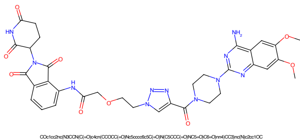
Figure 621: PROTAC - PROTAC ID: 2236
