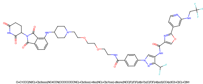
Figure 757: PROTAC - PROTAC ID: 1973
