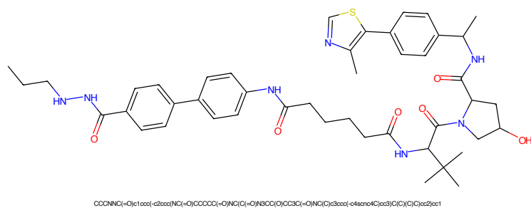
Figure 213: PROTAC - PROTAC ID: 2388
