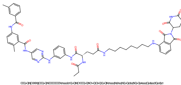
Figure 41: PROTAC - PROTAC ID: 415
