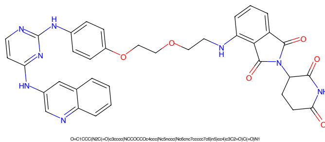
Figure 213: PROTAC - PROTAC ID: 1874
