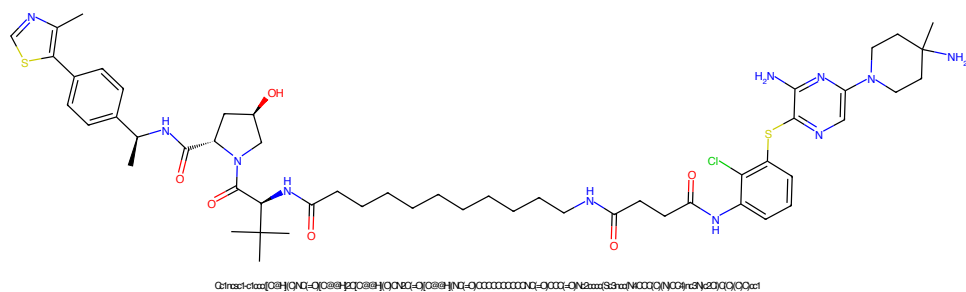
Figure 517: PROTAC - PROTAC ID: 2010
