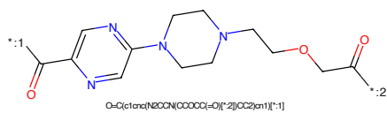
Figure 987: LINKER - PROTAC ID: 2291
