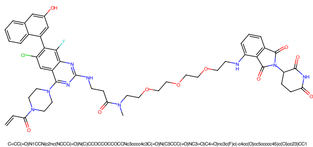
Figure 465: PROTAC - PROTAC ID: 1996
