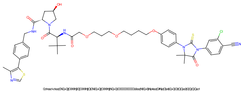
Figure 649: PROTAC - PROTAC ID: 2064
