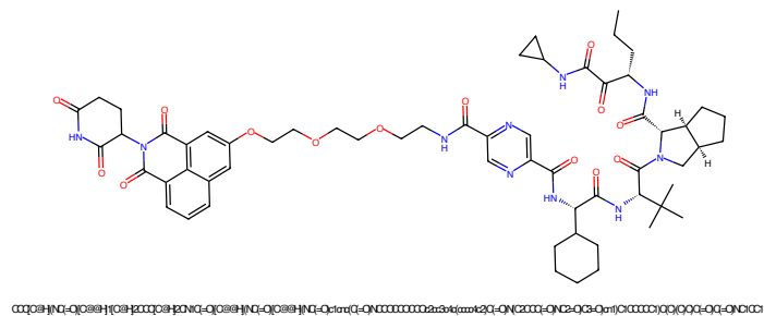
Figure 233: PROTAC - PROTAC ID: 1879
