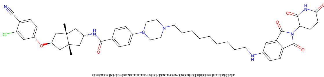
Figure 933: PROTAC - PROTAC ID: 2278
