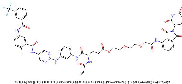
Figure 257: PROTAC - PROTAC ID: 1889
