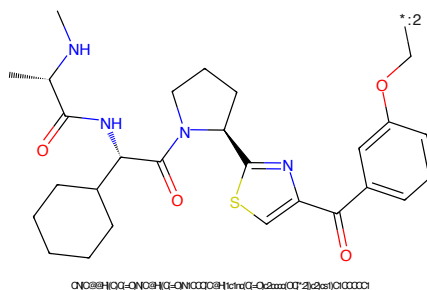
Figure 8: E3 - PROTAC ID: 1801
