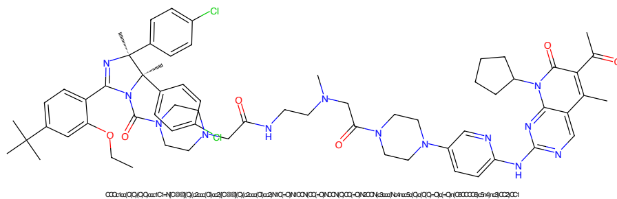
Figure 349: PROTAC - PROTAC ID: 1944
