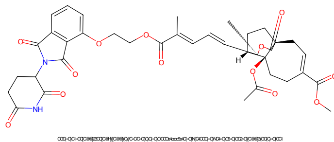
Figure 817: PROTAC - PROTAC ID: 2242
