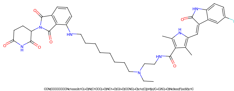
Figure 329: PROTAC - PROTAC ID: 1930
