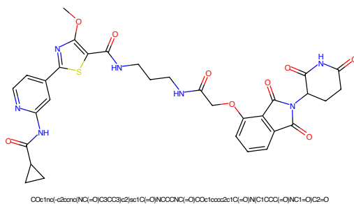
Figure 997: PROTAC - PROTAC ID: 2294
