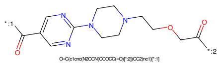
Figure 991: LINKER - PROTAC ID: 2292
