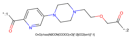
Figure 995: LINKER - PROTAC ID: 2293
