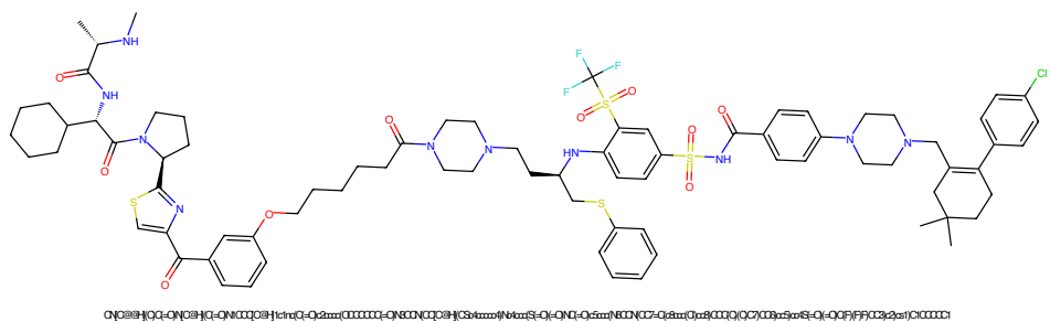
Figure 29: PROTAC - PROTAC ID: 1807
