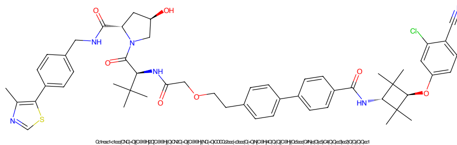
Figure 365: PROTAC - PROTAC ID: 1950
