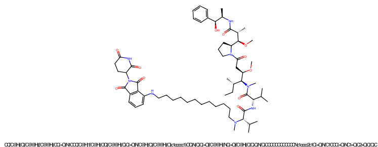
Figure 165: PROTAC - PROTAC ID: 1860
