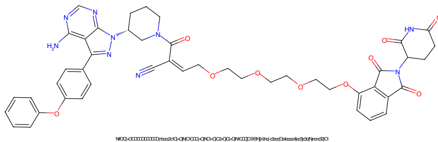
Figure 293: PROTAC - PROTAC ID: 1905
