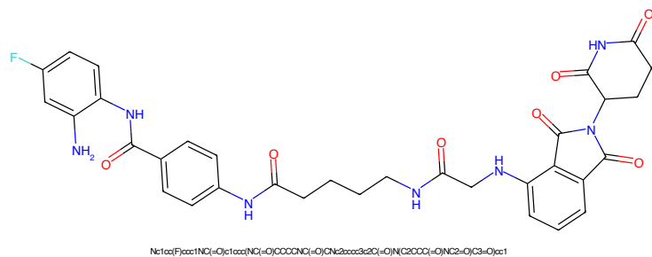
Figure 865: PROTAC - PROTAC ID: 2261
