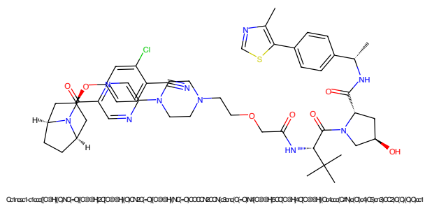
Figure 985: PROTAC - PROTAC ID: 2291
