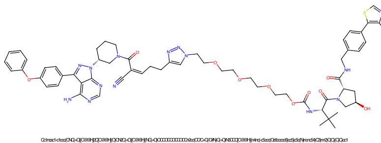
Figure 301: PROTAC - PROTAC ID: 1907
