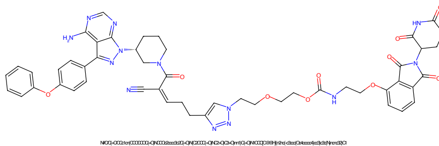
Figure 321: PROTAC - PROTAC ID: 1912
