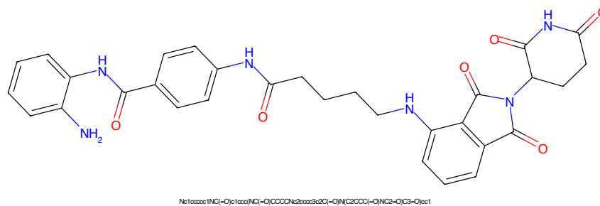
Figure 845: PROTAC - PROTAC ID: 2256
