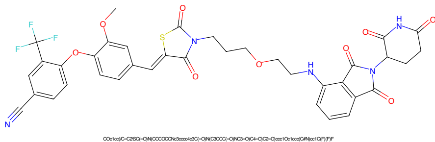
Figure 397: PROTAC - PROTAC ID: 1965
