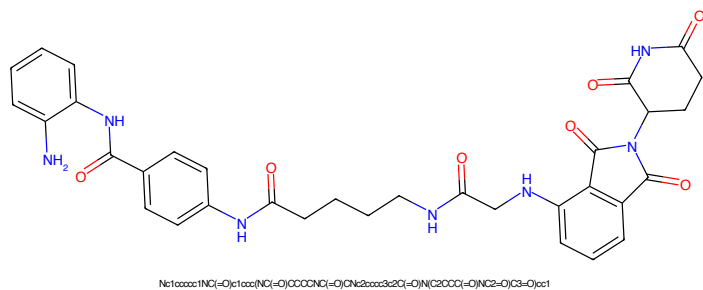
Figure 841: PROTAC - PROTAC ID: 2255
