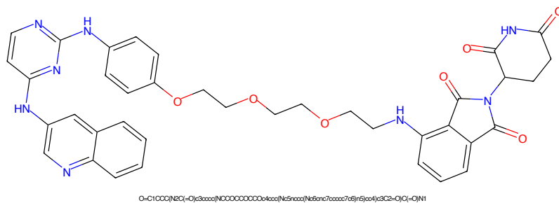
Figure 217: PROTAC - PROTAC ID: 1875
