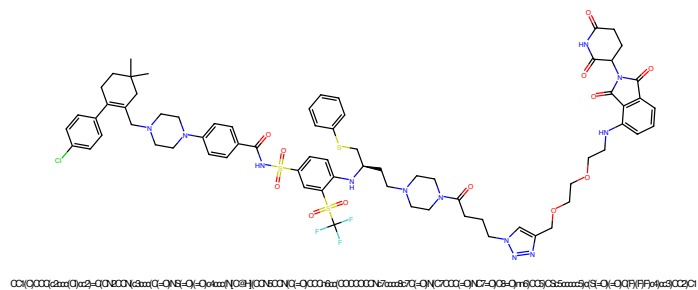
Figure 237: PROTAC - PROTAC ID: 1880
