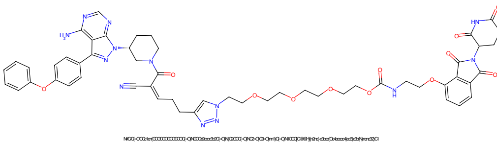
Figure 313: PROTAC - PROTAC ID: 1910
