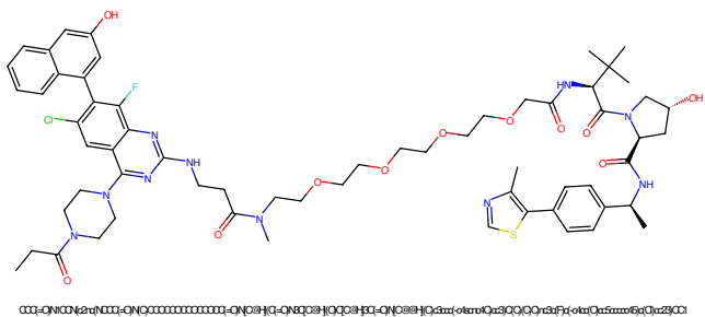
Figure 473: PROTAC - PROTAC ID: 1999
