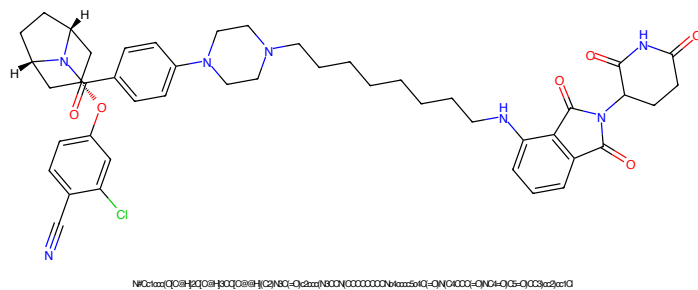
Figure 877: PROTAC - PROTAC ID: 2264
