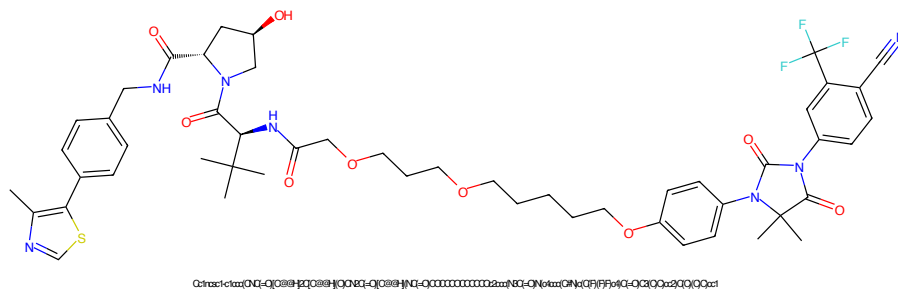
Figure 357: PROTAC - PROTAC ID: 1946
