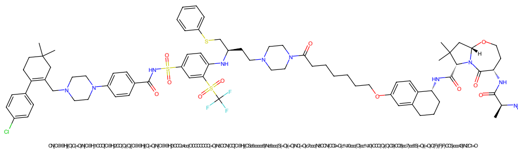
Figure 65: PROTAC - PROTAC ID: 1816
