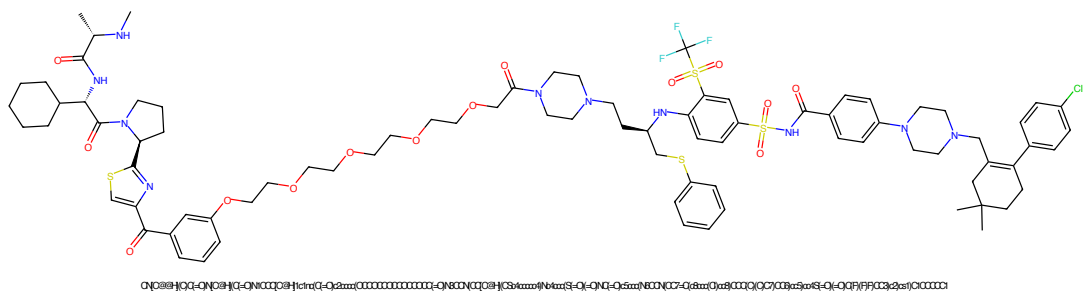
Figure 17: PROTAC - PROTAC ID: 1804
