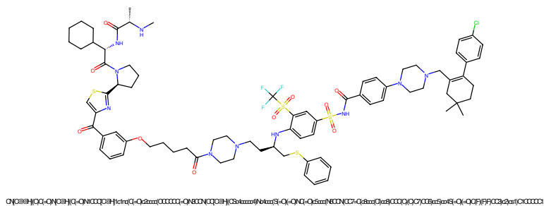
Figure 25: PROTAC - PROTAC ID: 1806
