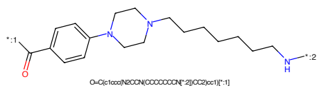
Figure 959: LINKER - PROTAC ID: 2284
