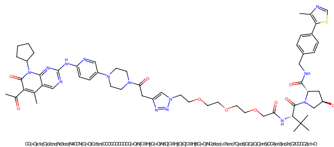
Figure 333: PROTAC - PROTAC ID: 1940
