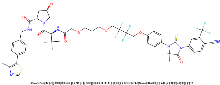
Figure 609: PROTAC - PROTAC ID: 2042
