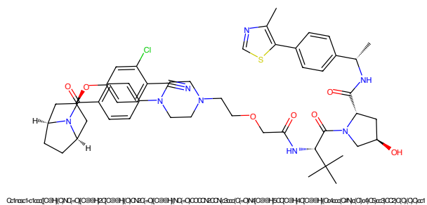
Figure 977: PROTAC - PROTAC ID: 2289
