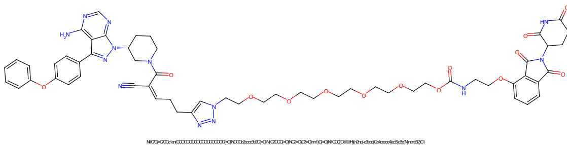
Figure 325: PROTAC - PROTAC ID: 1913
