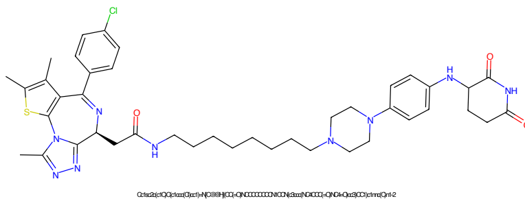
Figure 369: PROTAC - PROTAC ID: 1957
