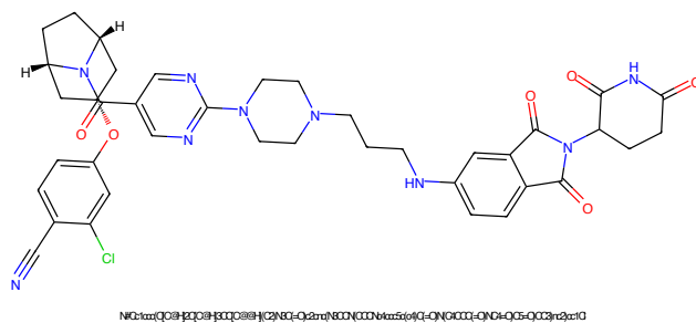
Figure 917: PROTAC - PROTAC ID: 2274
