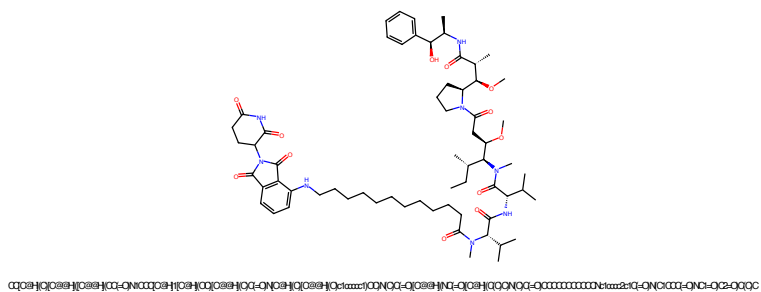
Figure 169: PROTAC - PROTAC ID: 1861
