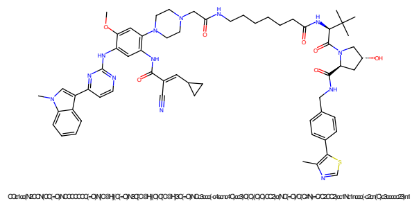
Figure 433: PROTAC - PROTAC ID: 2986
