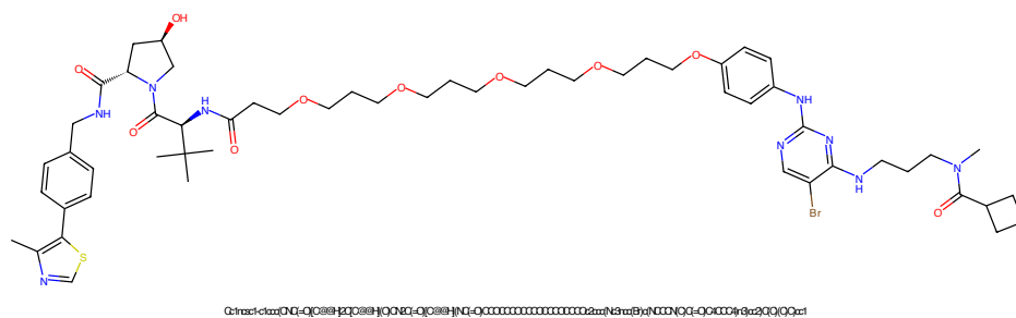
Figure 469: PROTAC - PROTAC ID: 172
