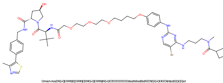
Figure 445: PROTAC - PROTAC ID: 166
