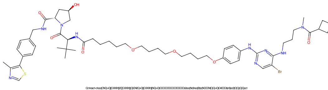
Figure 457: PROTAC - PROTAC ID: 169
