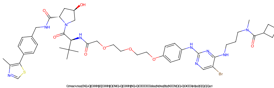
Figure 425: PROTAC - PROTAC ID: 161
