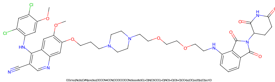
Figure 417: PROTAC - PROTAC ID: 158
