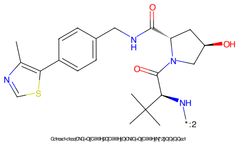
Figure 224: E3 - PROTAC ID: 60
