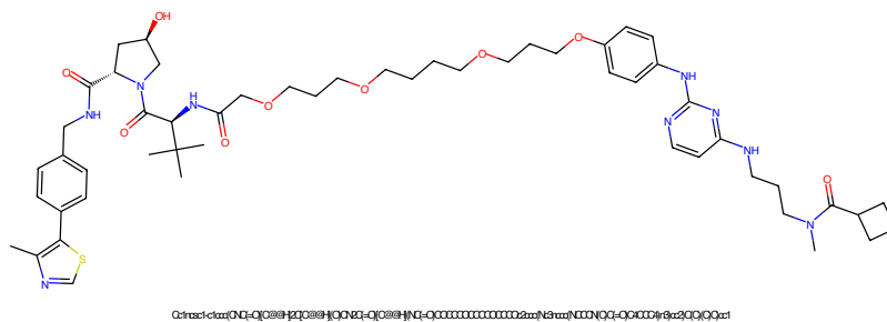
Figure 485: PROTAC - PROTAC ID: 176
