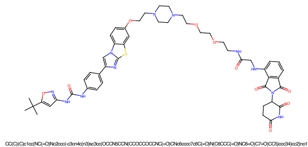
Figure 409: PROTAC - PROTAC ID: 156
