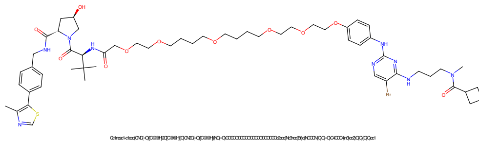
Figure 477: PROTAC - PROTAC ID: 174
