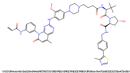
Figure 237: PROTAC - PROTAC ID: 70
