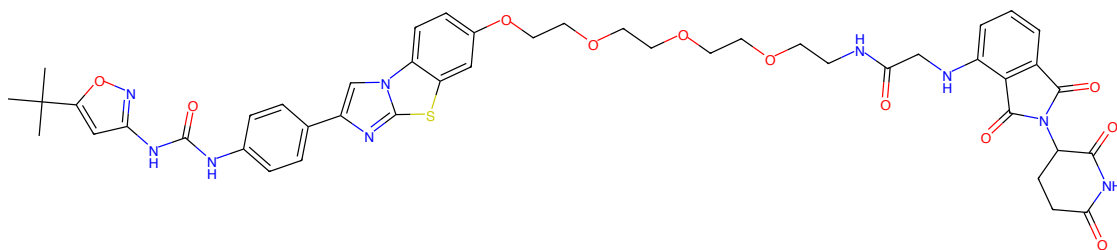
Figure 413: PROTAC - PROTAC ID: 157
