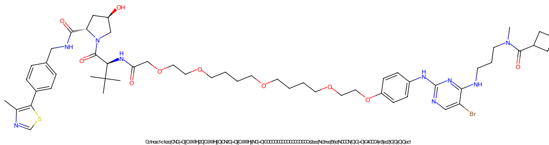
Figure 465: PROTAC - PROTAC ID: 171
