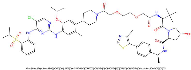
Figure 13: PROTAC - PROTAC ID: 1992
