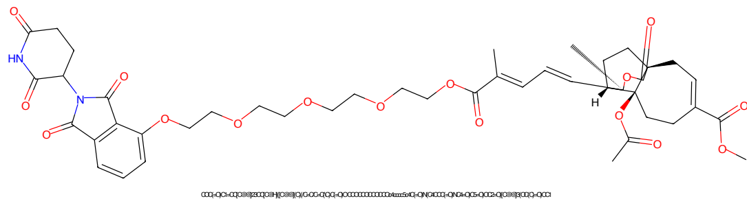
Figure 365: PROTAC - PROTAC ID: 2247
