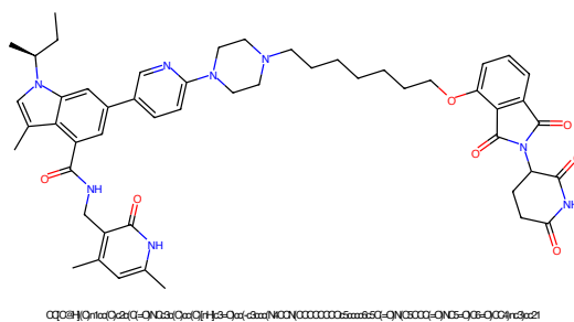
Figure 265: PROTAC - PROTAC ID: 2177
