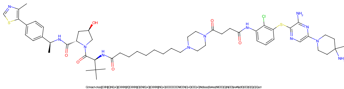
Figure 117: PROTAC - PROTAC ID: 2019
