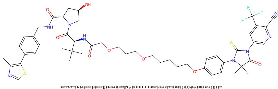
Figure 177: PROTAC - PROTAC ID: 2059
