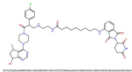
Figure 5: PROTAC - PROTAC ID: 2942
