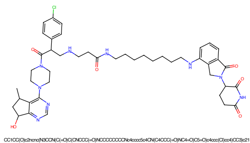
Figure 13: PROTAC - PROTAC ID: 2944
