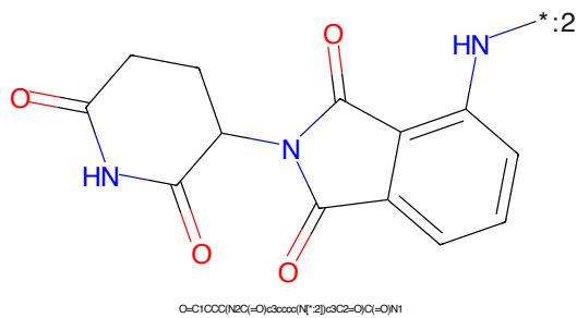
Figure 4: E3 - PROTAC ID: 2941
