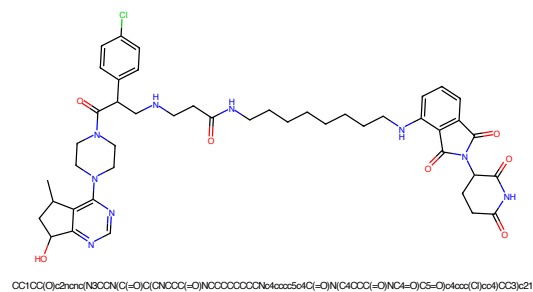
Figure 1: PROTAC - PROTAC ID: 2941
