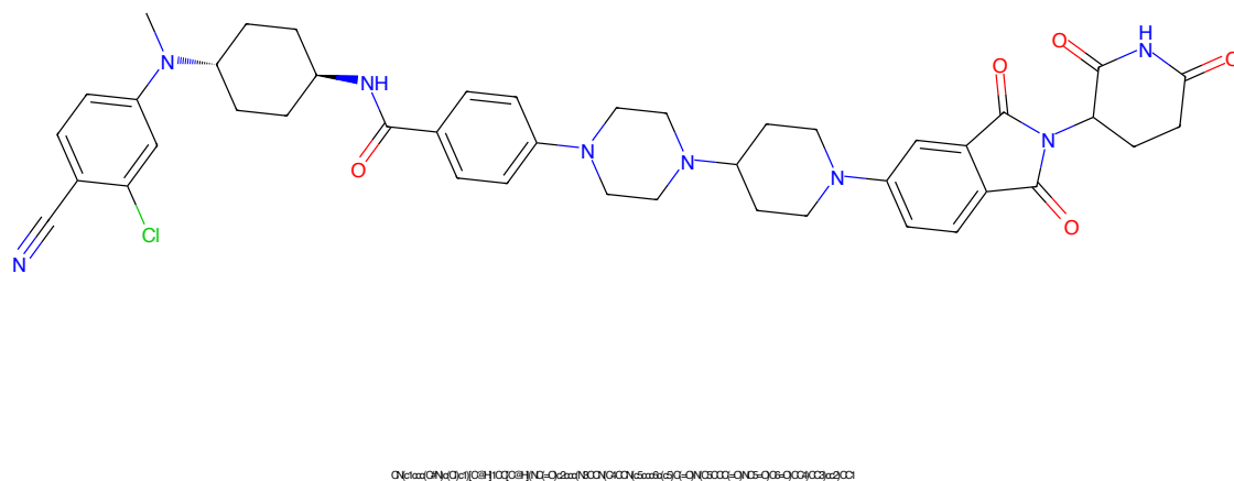
Figure 36: PROTAC ID: 2895
