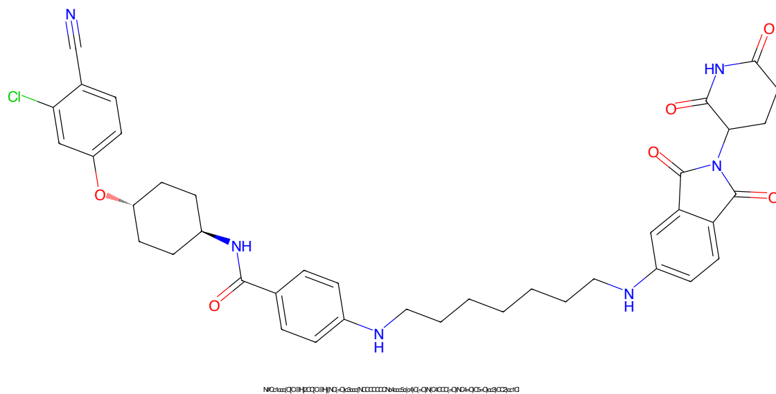
Figure 35: PROTAC ID: 2870
