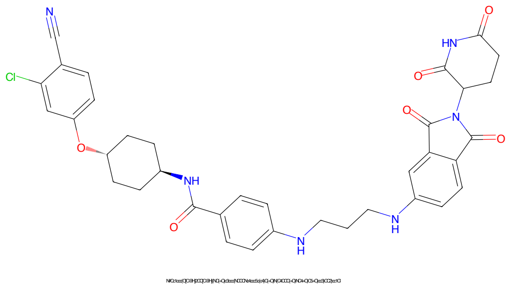
Figure 69: PROTAC ID: 2866
