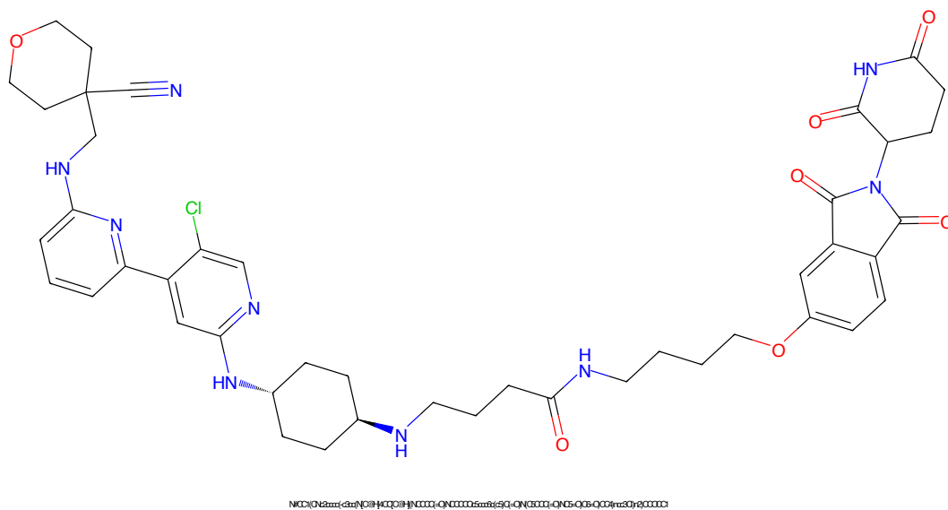
Figure 123: PROTAC ID: 248
