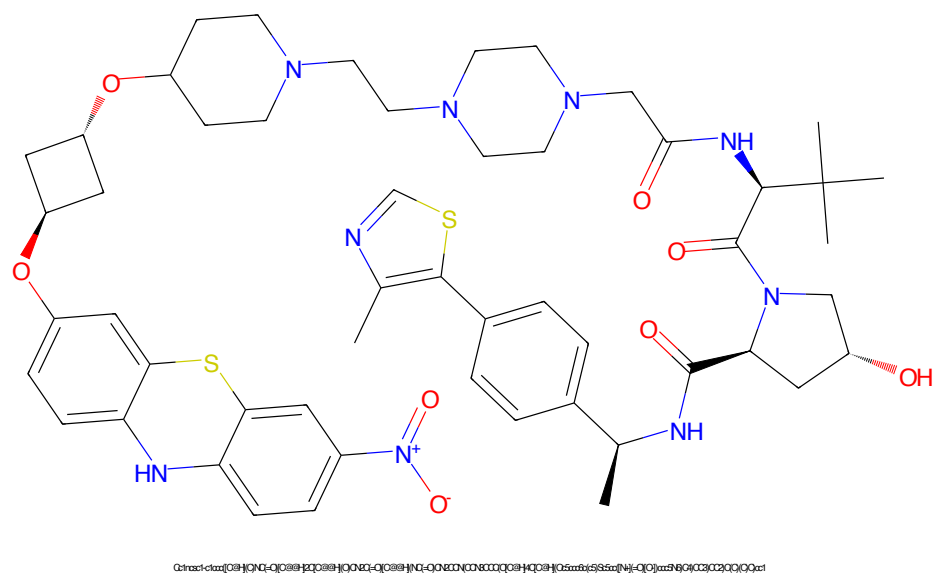
Figure 95: PROTAC ID: 2050
