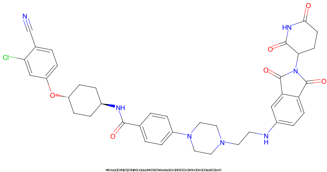
Figure 39: PROTAC ID: 2875
