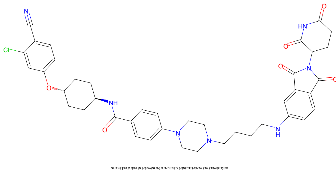
Figure 101: PROTAC ID: 2877
