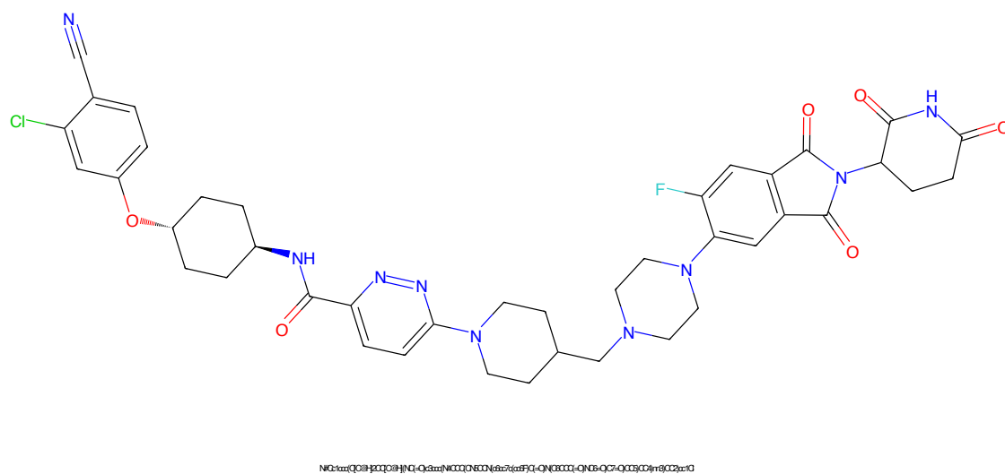
Figure 43: PROTAC ID: 3640
