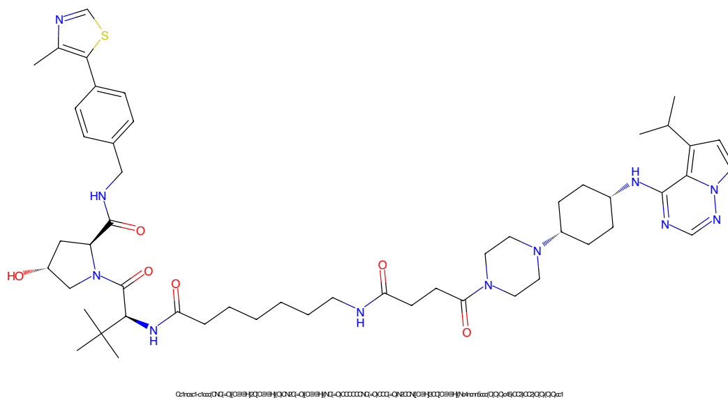
Figure 92: PROTAC ID: 2125
