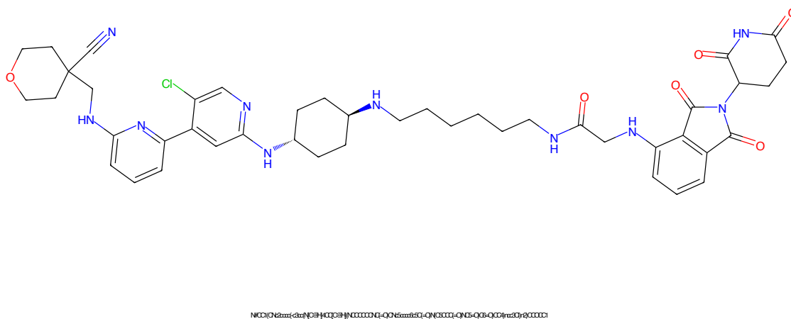
Figure 124: PROTAC ID: 247
