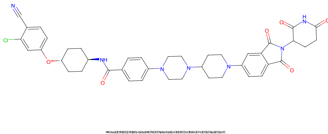
Figure 93: PROTAC ID: 2880
