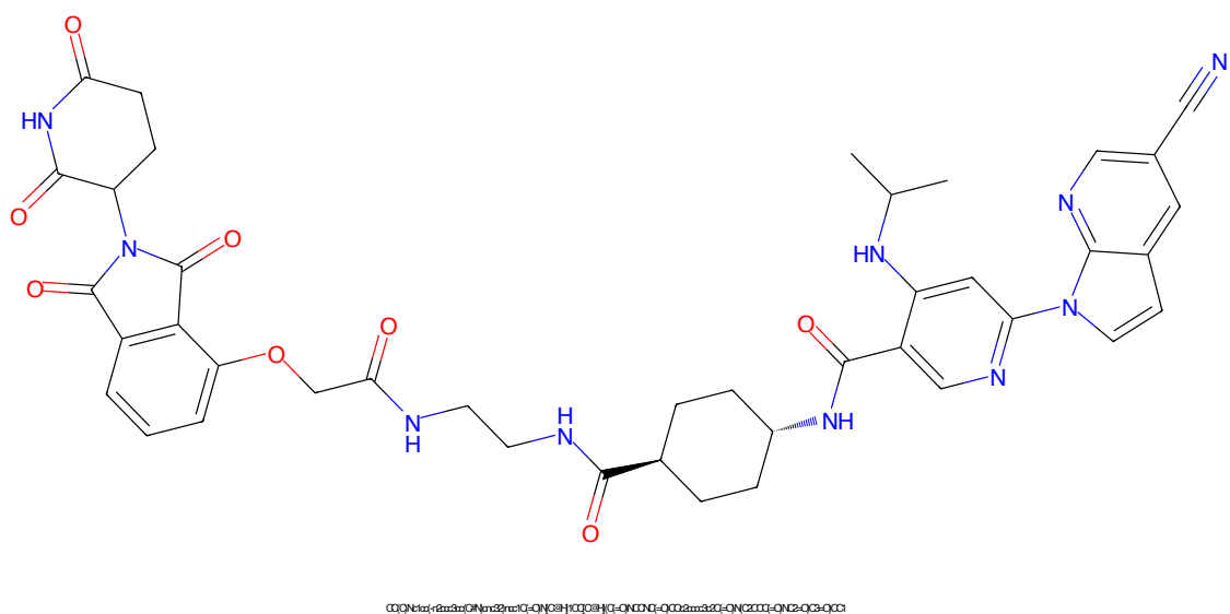
Figure 70: PROTAC ID: 2376
