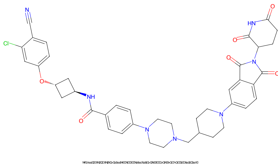
Figure 94: PROTAC ID: 2705
