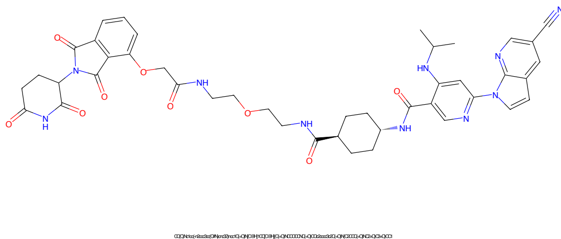
Figure 96: PROTAC ID: 2380
