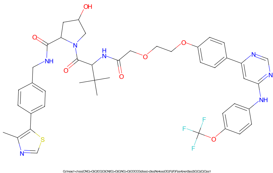
Figure 40: PROTAC ID: 1628
