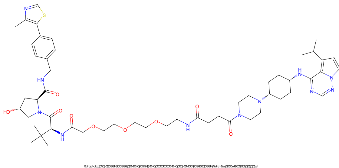
Figure 102: PROTAC ID: 2122
