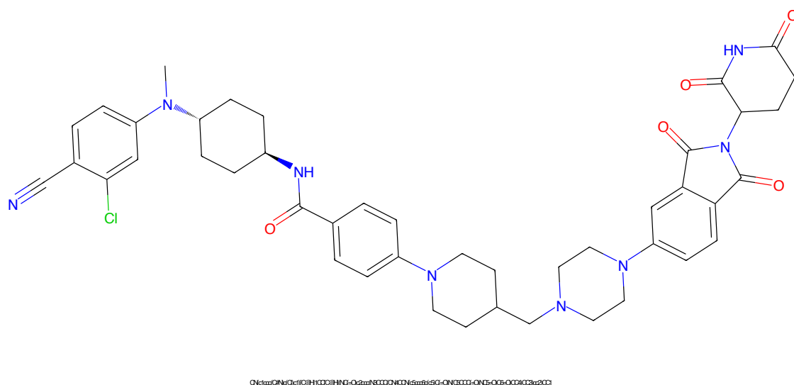
Figure 91: PROTAC ID: 2894
