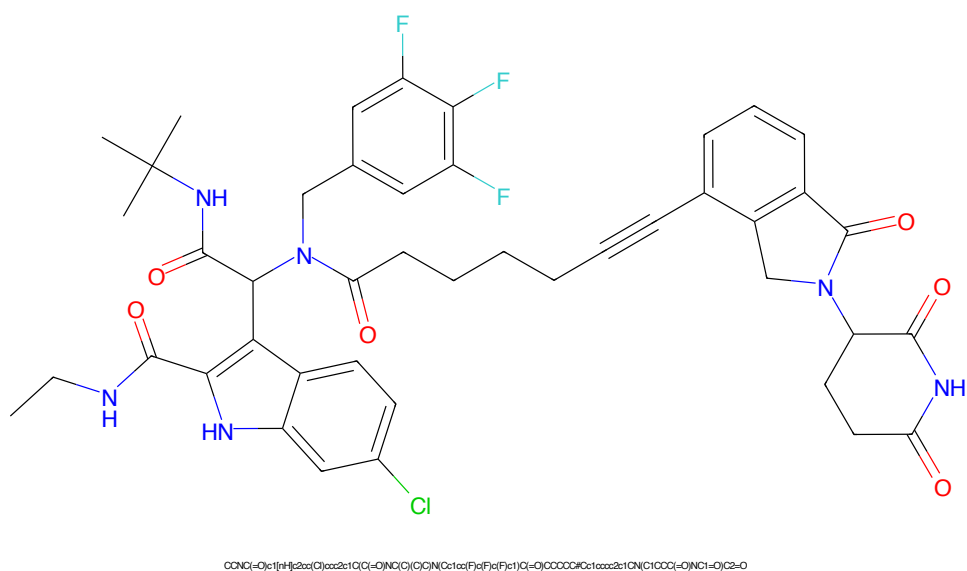
Figure 44: PROTAC ID: 3178
