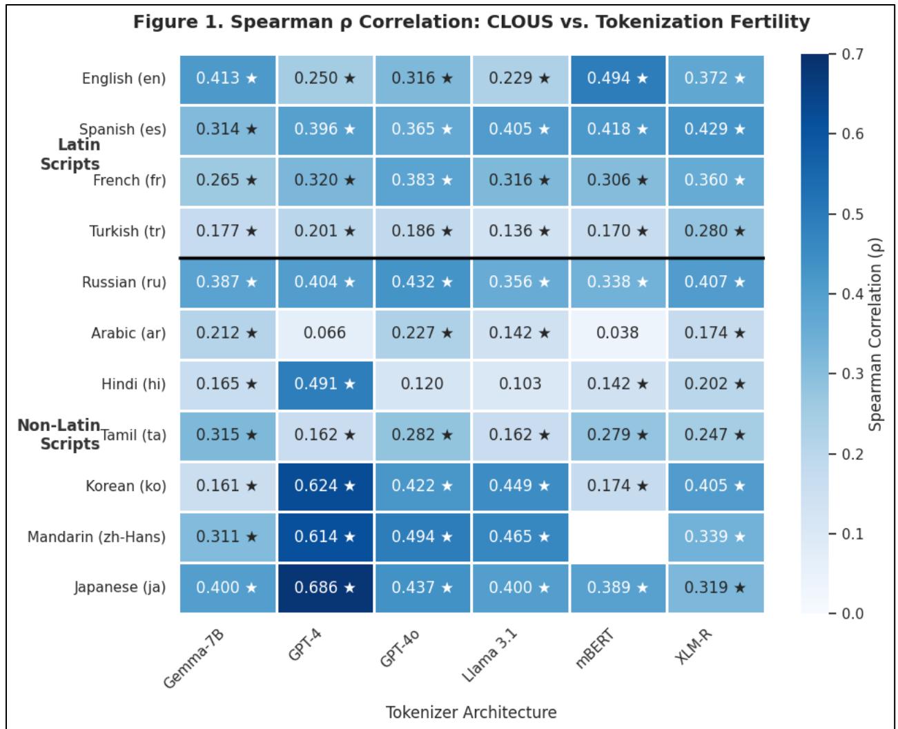
Figure 1: Spearman \rho between CLOUS scores and tokenization fertility across all language-tokenizer combinations.
