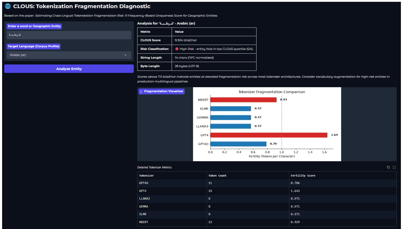
Figure C1: The web interface for the CLOUS Tokenizer Diagnostic tool, demonstrating the risk classification and tokenization analysis for the elongated Arabic entity قربطبة.
