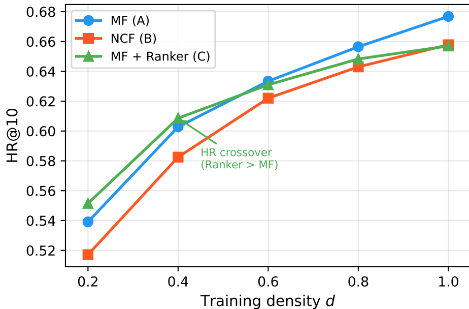
HR@10 vs. Training Density
