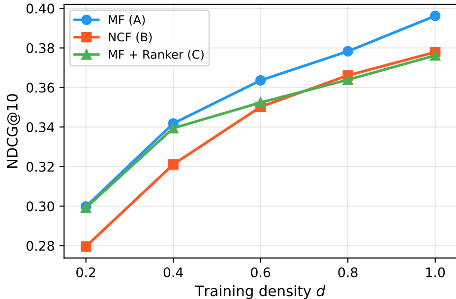
NDCG@10 vs. Training Density
