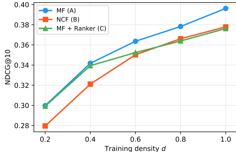
Ranking Quality (NDCG@10)
