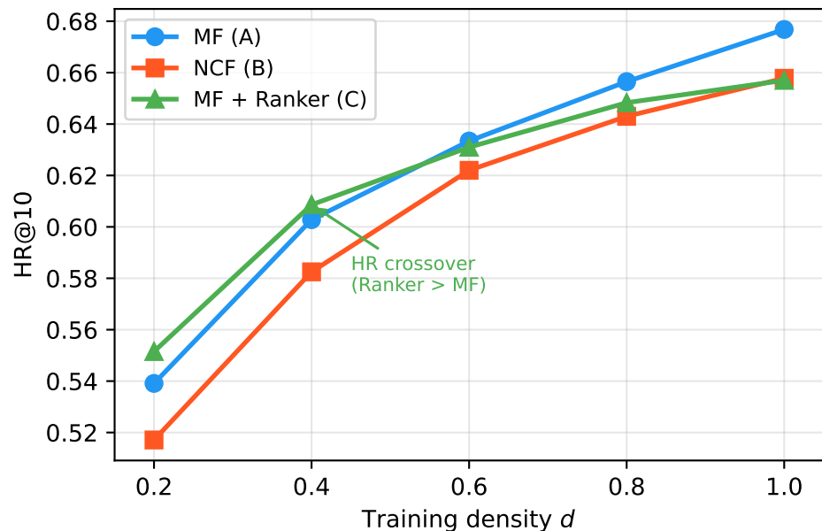
Hit Rate (HR@10)
