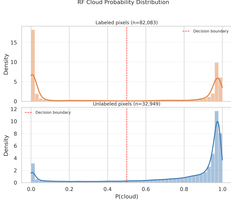
Figure 21: RF cloud probability distributions for labeled (top) and unlabeled (bottom) pixels in orbit 0013490, shown in separate panels with a shared x-axis. Smooth curves are Gaussian KDE estimates ( h = 0.05\hat{\sigma} , narrow bandwidth chosen to preserve the sharp bimodal peaks).
