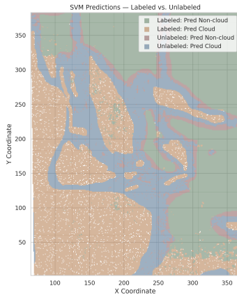
Figure 19: SVM(Lit) spatial map
