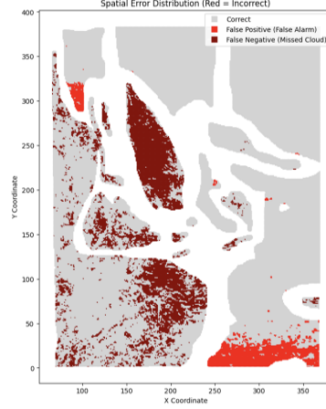
Figure 15: Spatial map of classification errors in the Stepwise Logistic Regression model.
