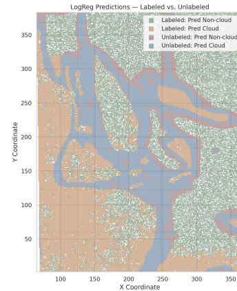
Figure 20: Stepwise Logistic Regression
