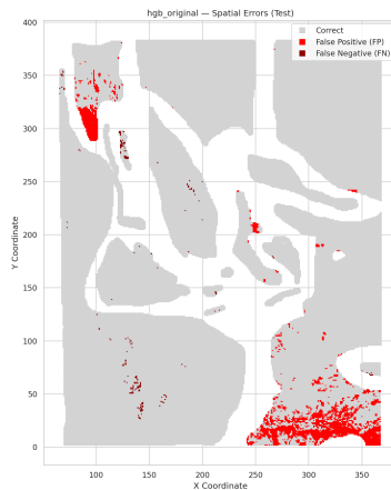
Figure 12: Spatial map of classification errors concentrated at cloud edges.
