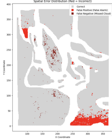
Figure 14: Spatial map of classification errors in the SVM (Lit) model setting.
