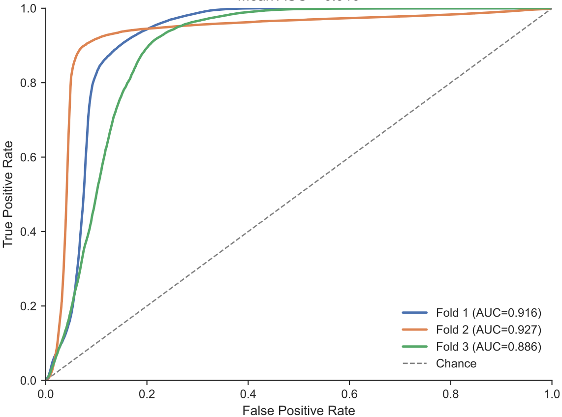
ROC Curves for Best LDA Mean AUC = 0.910
