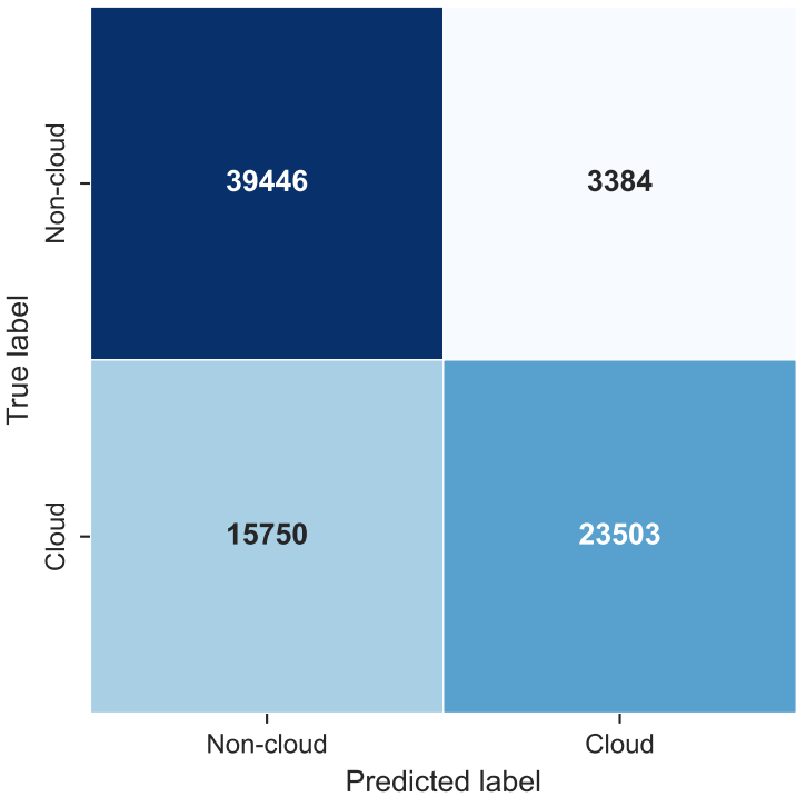
Confusion Matrix (Fold 1)
