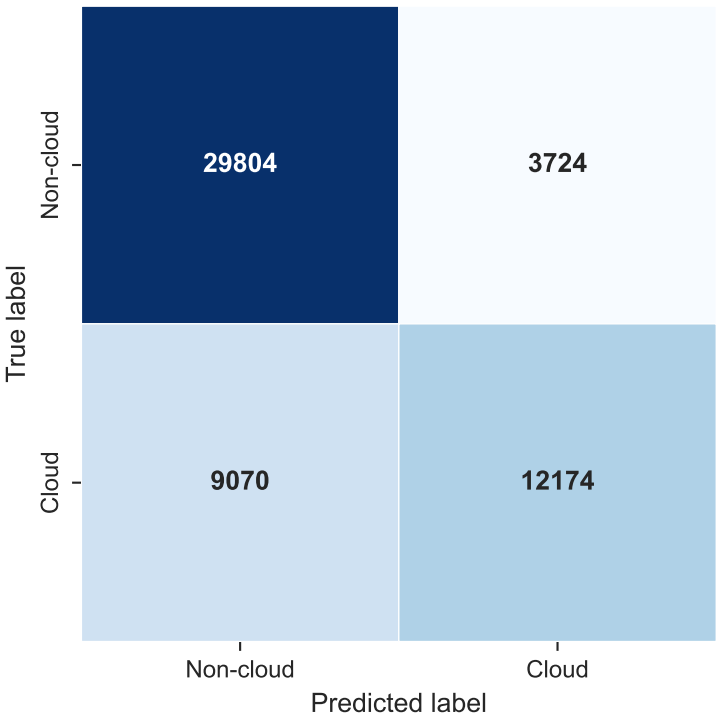
Confusion Matrix (Fold 3)
