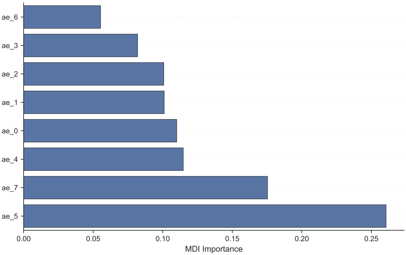
Feature Importance from Random Forest (MDI)
