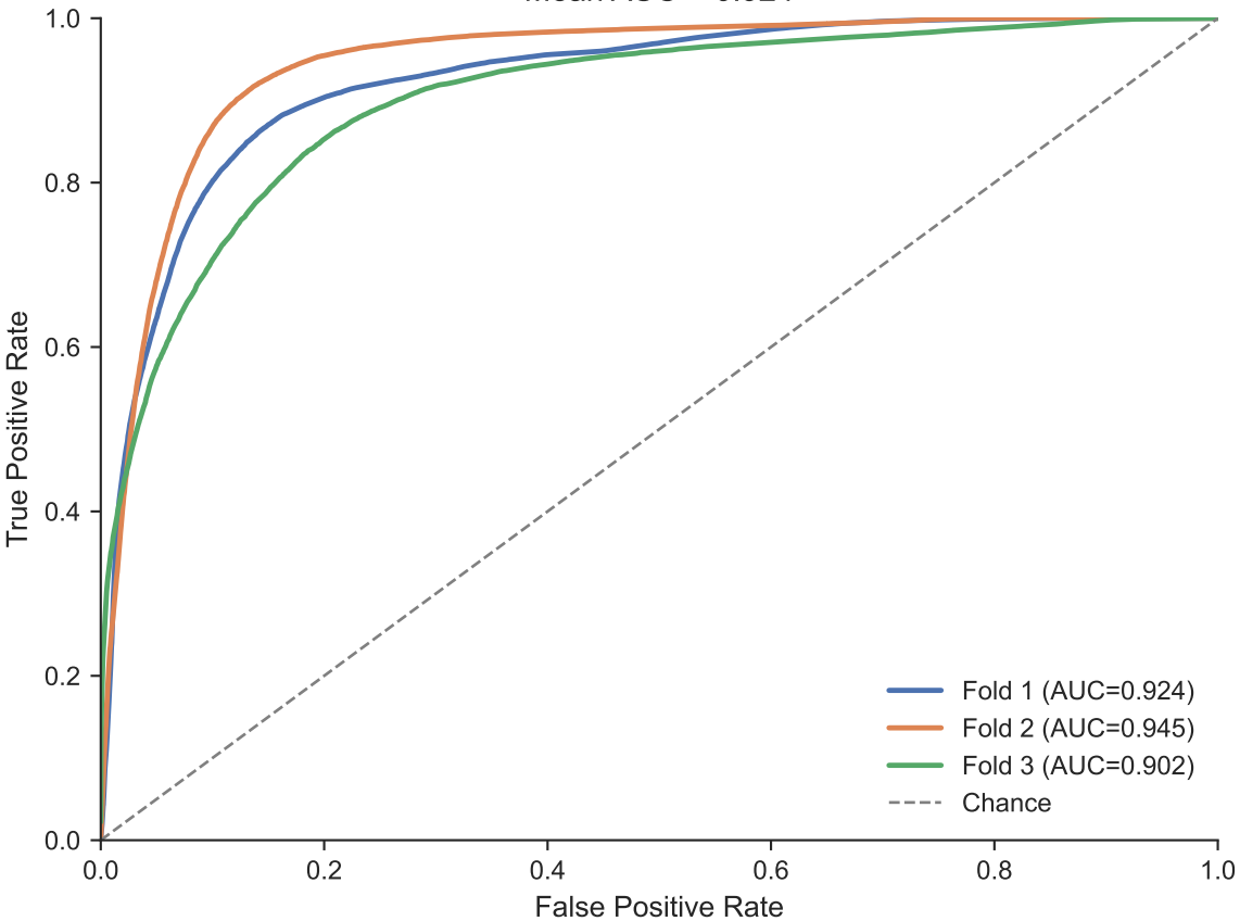
ROC Curves for Best Random Forest Mean AUC = 0.924
