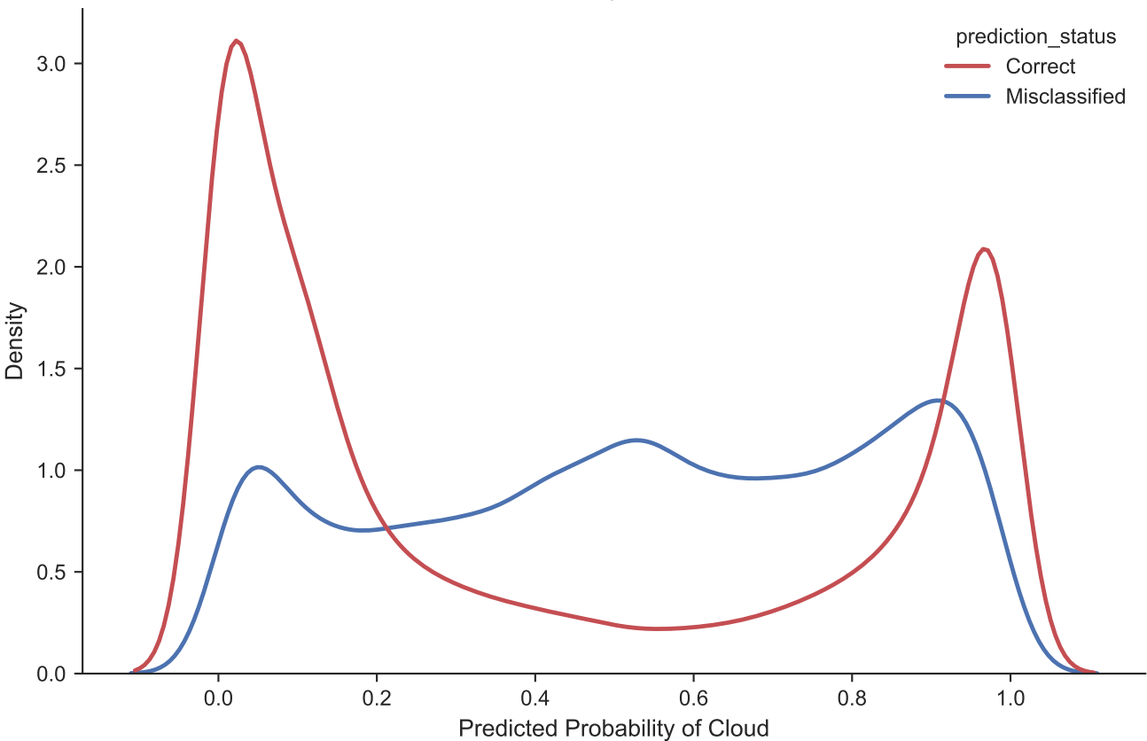
Prediction Confidence by Classification Outcome
