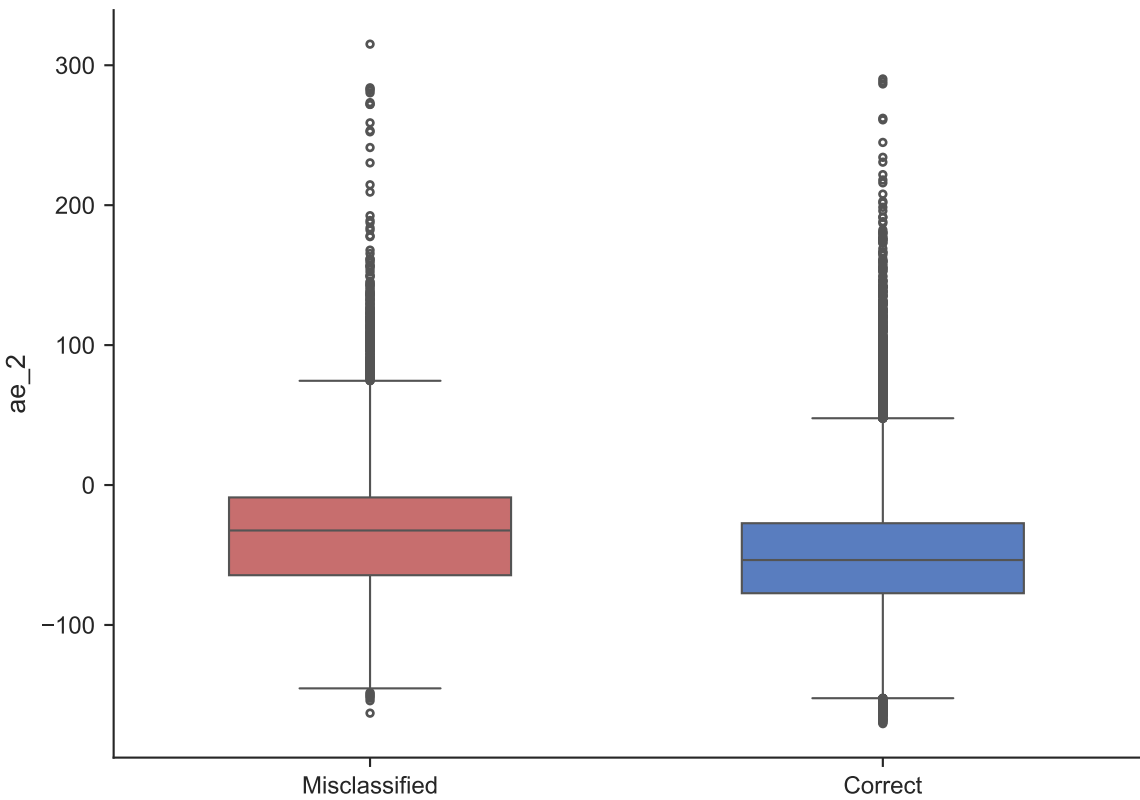
ae_2 Distribution: Correct vs Misclassified
