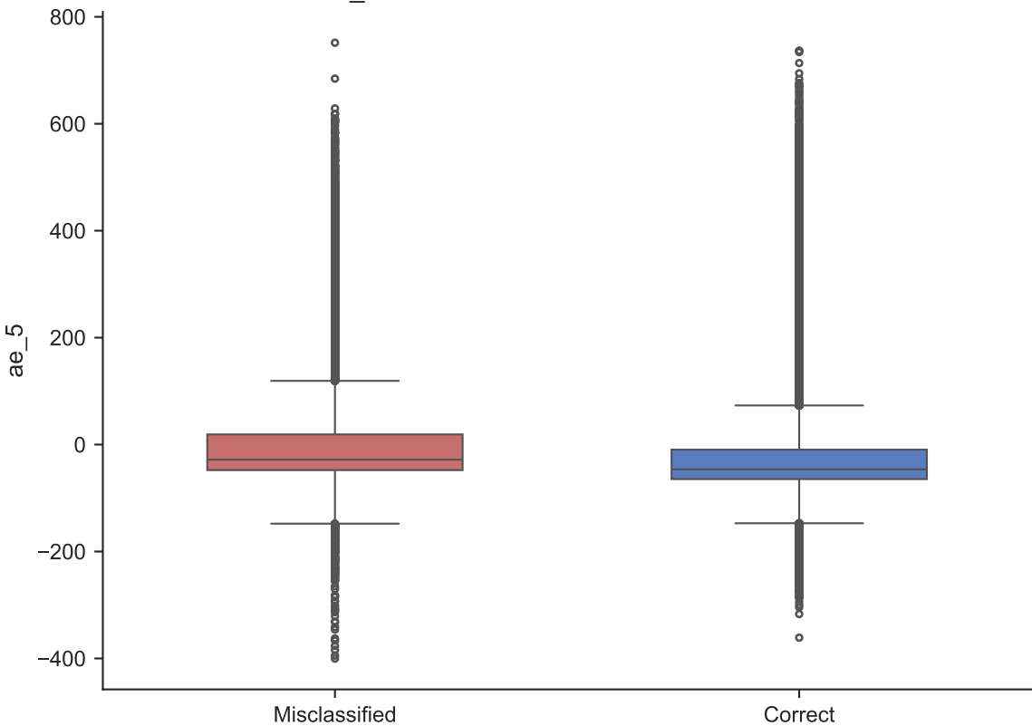
ae_5 Distribution: Correct vs Misclassified
