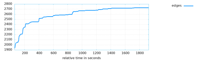
Figure 2: Baseline QEMU decoder edges over time.
