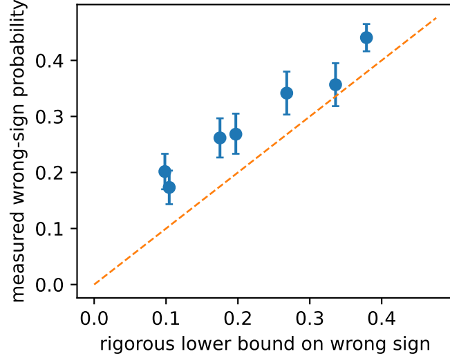
(c) Final-fidelity bound
