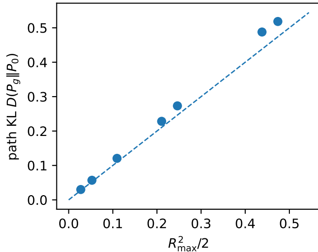
(b) KZ information action
