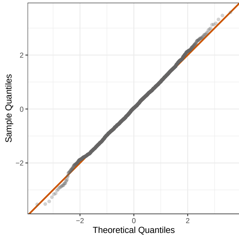
A – QQ plot
