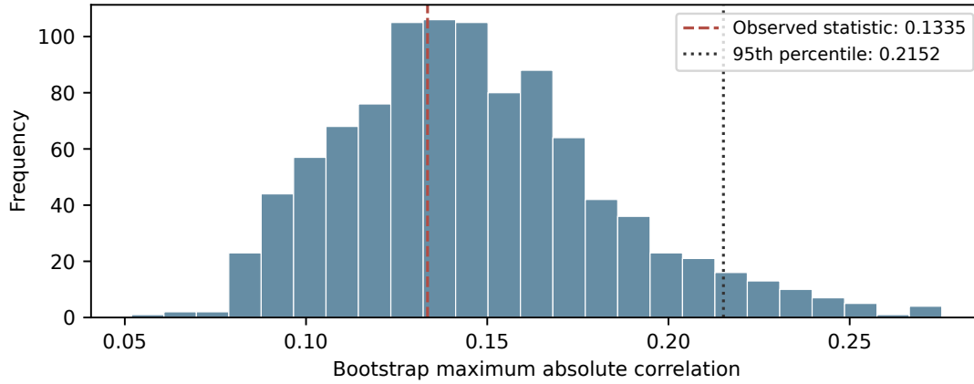
Figure 3: Bootstrap maximum-statistic distribution for the first null trial. The observed statistic is 0.1335; the empirical 95th percentile is 0.2152.
