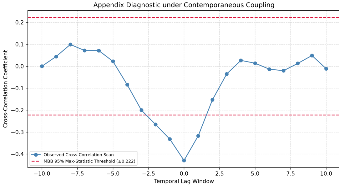
Figure 5: Illustrative scan under Y_t = -0.3X_t + U_t . The contemporaneous coupling induces correlation at neighboring lags. Dashed lines show the MBB maximum-statistic threshold (approximately \pm 0.222 ) under process independence.
