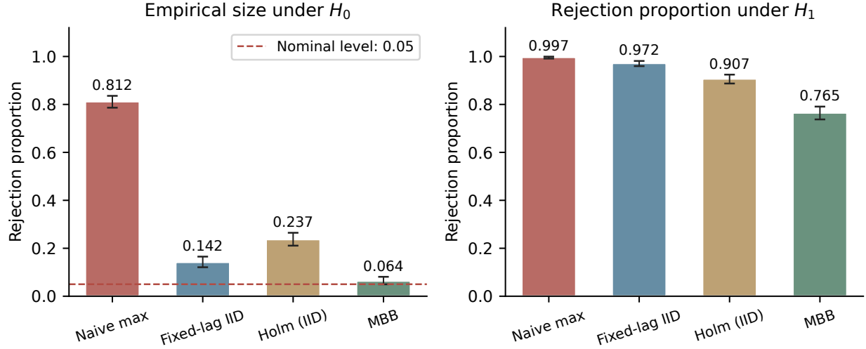
Figure 2: Rejection proportions under the null and alternative. Error bars are exact 95% binomial intervals; the dashed line marks the nominal 0.05 level.
