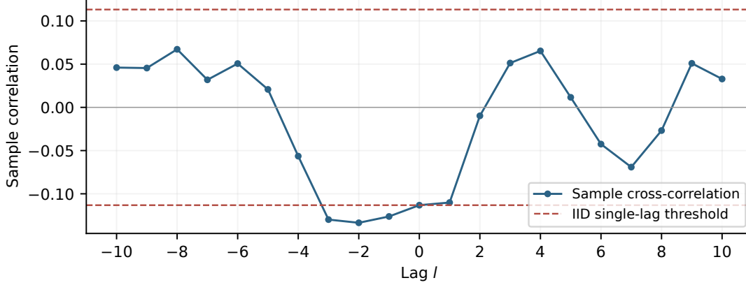
Figure 1: Lag scan for the first independent AR(1) null trial. The dashed lines mark the IID single-lag threshold.
