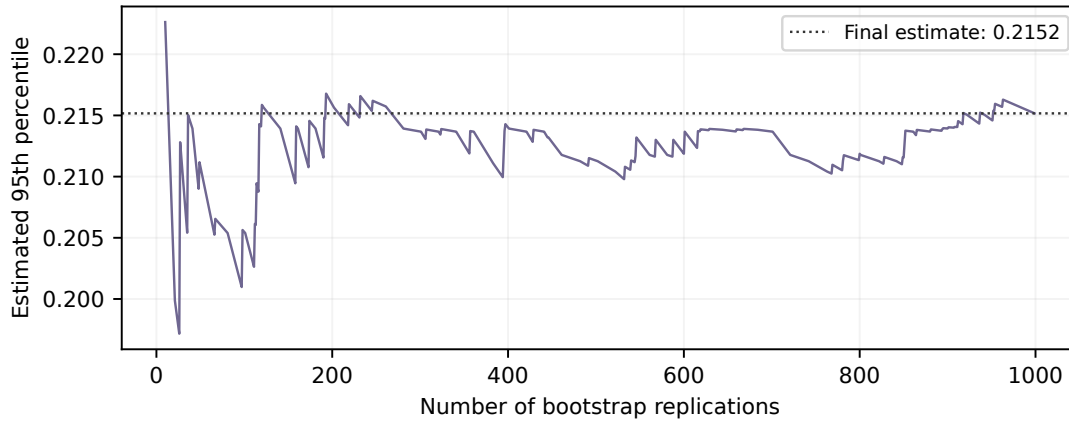
Figure 4: Running estimate of the bootstrap 95th percentile for the first null trial.
