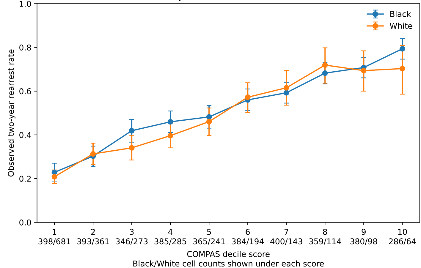
Observed two-year rearrest rate within each score
