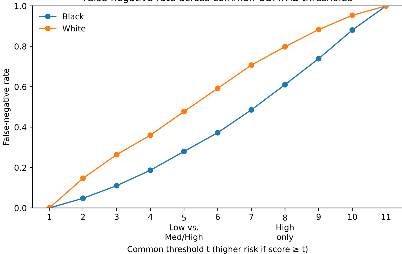
False-negative rate across common COMPAS thresholds
