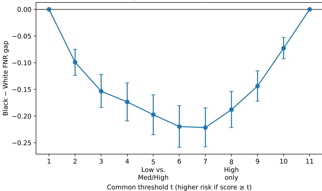
Black – White FNR gap across thresholds 95% pointwise bootstrap intervals
