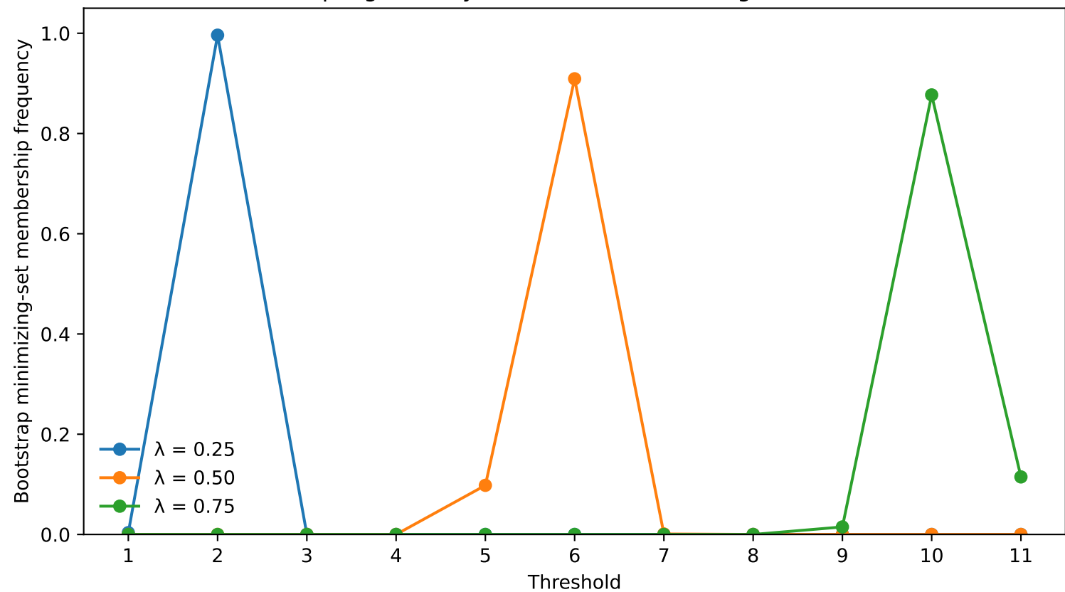
Sampling stability of focal loss-minimizing thresholds
